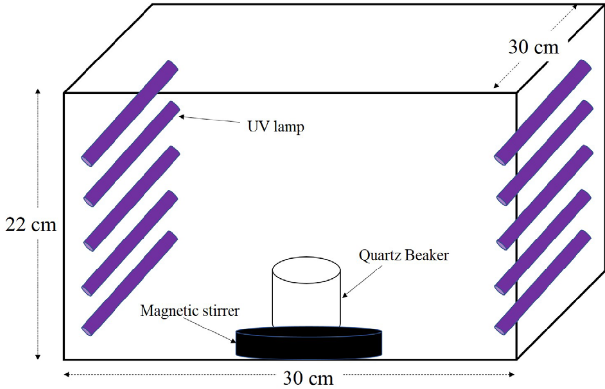
Figure S1 Diagram of the photoreactor
