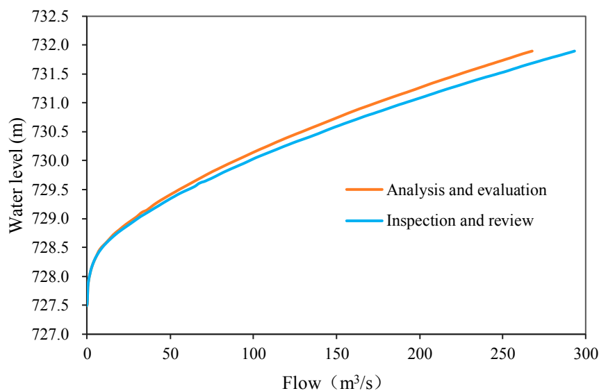
Figure 5. Water level flow relationship of Shangqing-4.
