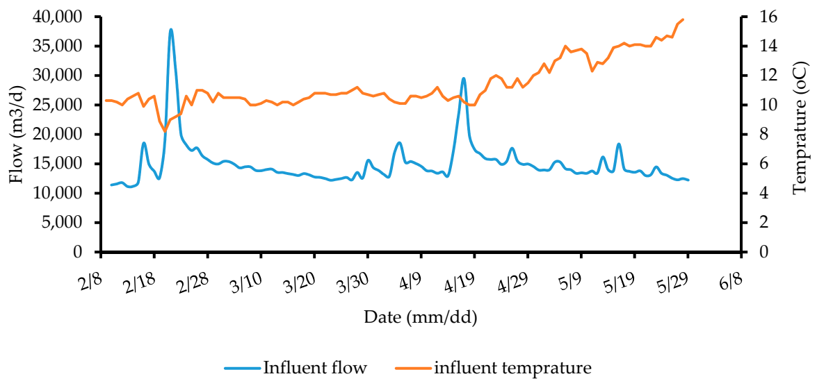
Figure S1. Seasonal changes in influent flow rate and temperature of Vauxhall WWTP.
