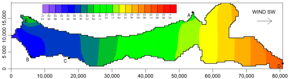
Figure 13. Water surface elevation (m a.s.l.) after 12 h of a SW wind at a speed of 12 \text{ m s}^{-1} and with the new artificial strait at point E (dimensions in meters).
