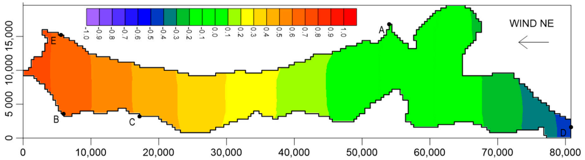
Figure 7. Water surface elevation (m a.s.l.) after 12 h of a NE wind at a speed of 12 \text{ m s}^{-1} and without the new artificial strait at point E (dimensions in meters).
