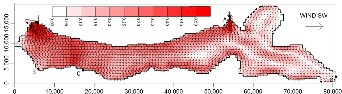
Figure 14. Water flow velocity ( \text{m s}^{-1} ) after 12 h of a SW wind at a speed of 12 \text{ m s}^{-1} and with the new artificial strait at point E (dimensions in meters).
