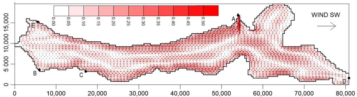
Figure 12. Water flow velocity ( \text{m s}^{-1} ) after 12 h of a SW wind at a speed of 12 \text{ m s}^{-1} and without the new artificial strait at point E (dimensions in meters).
