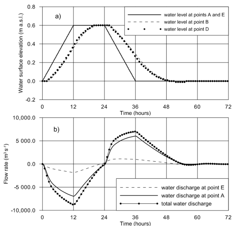
Figure 6. (a) Imposed boundary conditions (points A–Baltiysk and E–Nowy Świat), and calculated water levels (points B–Nowakowo and D–Kaliningrad) and (b) calculated water discharges at point A in the Strait of Baltiysk and at point E in the new canal (Nowy Świat).
