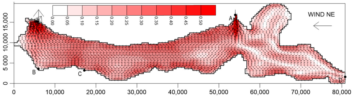
Figure 10. Water flow velocity ( \text{m s}^{-1} ) after 12 h of a NE wind at a speed of 12 \text{ m s}^{-1} and with the new artificial strait at point E (dimensions in meters).
