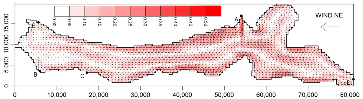
Figure 8. Water flow velocity ( \text{m s}^{-1} ) after 12 h of a NE wind at a speed of 12 \text{ m s}^{-1} and without the new artificial strait at point E (dimensions in meters).
