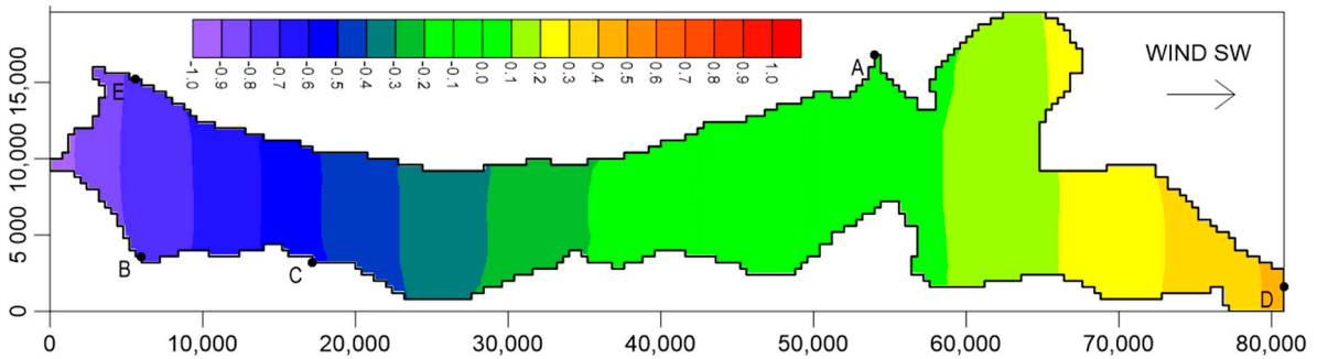
Figure 11. Water surface elevation (m a.s.l.) after 12 h of a SW wind at a speed of 12 \text{ m s}^{-1} and without the new artificial strait at point E (dimensions in meters).
