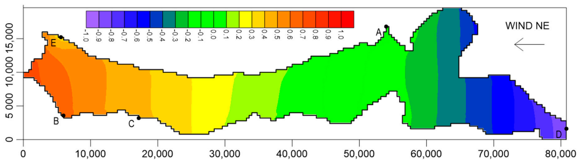
Figure 9. Water surface elevation (m a.s.l.) after 12 h of a NE wind at a speed of 12 \text{ m s}^{-1} and with the new artificial strait at point E (dimensions in meters).
