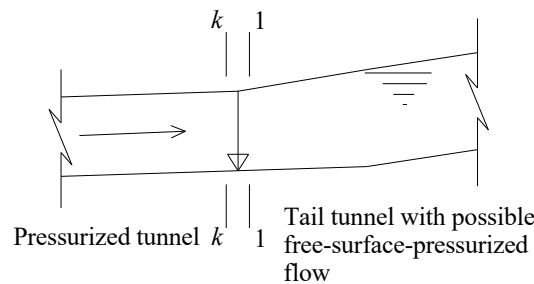
Figure 2. Inlet section of a tail tunnel with free-surface-pressurized flow.
