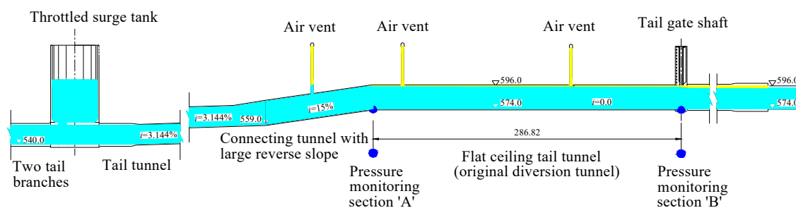
Figure 5. Layout of the tail system.
