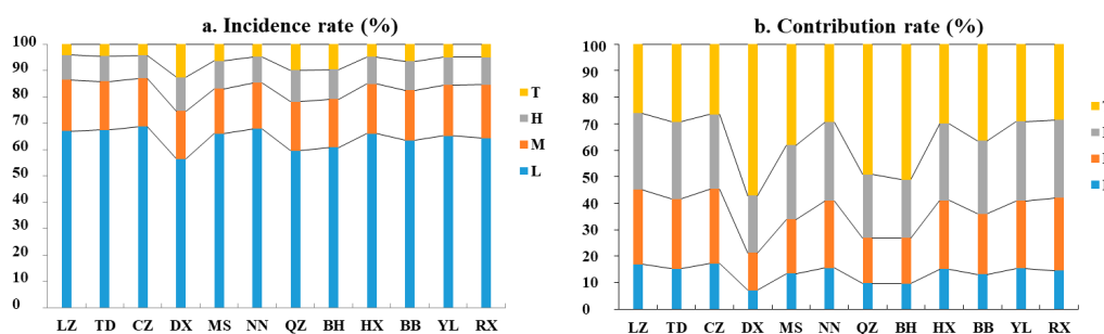
Figure 6. Incidence rate (a) and contribution rate (b) of different precipitation grades in rainy season at 12 stations in the Beibu Gulf.
