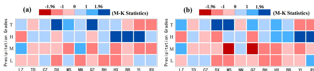
Figure 9. Variation tendency of incidence rate (a) and contribution rate of different grades (b) in rainy season at 12 stations in the Beibu Gulf. The letters along the y-axis denoted precipitation grades. L is Light rain, M is Moderate rain, H is Heavy rain and T is Torrential rain. The letters along the x-axis denoted names of the precipitation stations: Longzhou (LZ), Tiandeng (TD), Chongzuo (CZ), Dongxing (DX), Mashan (MS), Nanning (NN), Qinzhou (QZ), Beihai (BH), Hengxian (HX), Bobai (BB), Yulin (YL), and Rongxian (RX).
