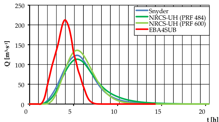
Figure 5. Design hydrograph for T = 500 years return period.
