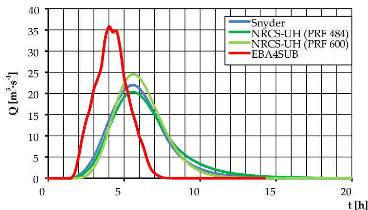
Figure 7. Design hydrograph for T = 10 years return period.
