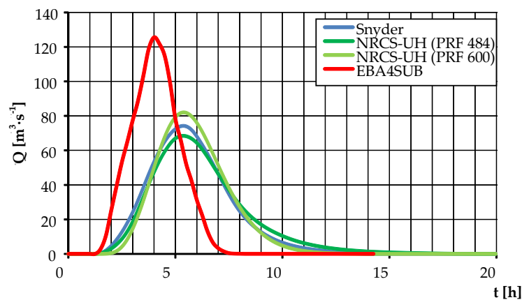
Figure 6. Design hydrograph for T = 100 years return period.
