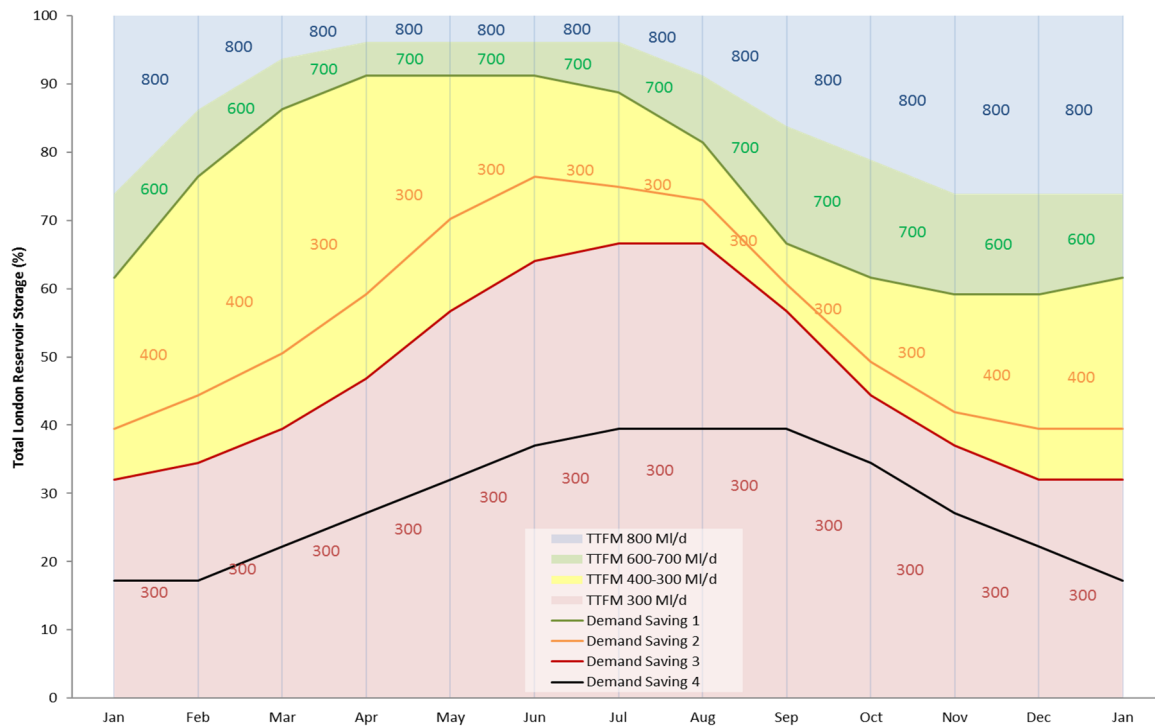
Figure 1. The Lower Thames Control Diagram (LTCD).
