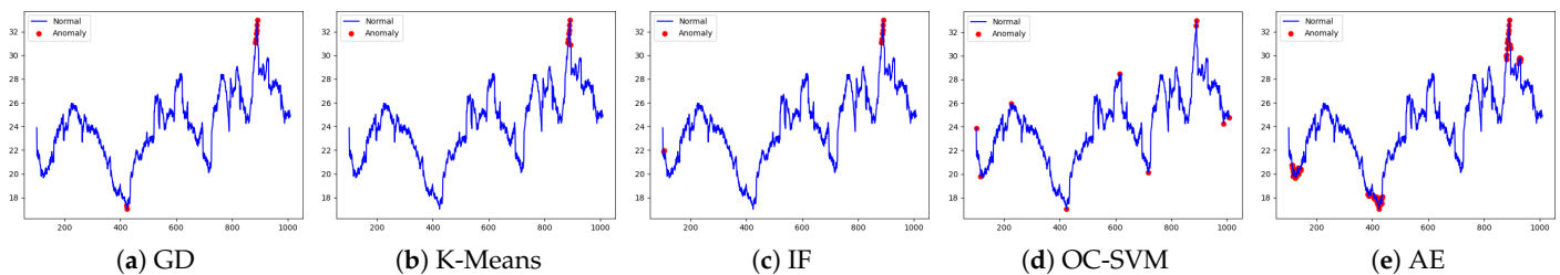
Figure 2. Anomaly Detection (Note: the line is the time series and the dot is the anomaly).
