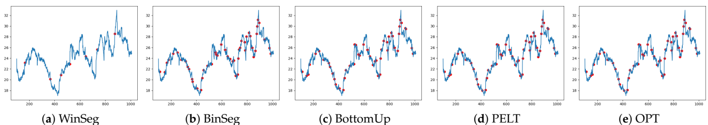
Figure 3. Change Point Detection (Note the line is the time series and the dot is the change point).
