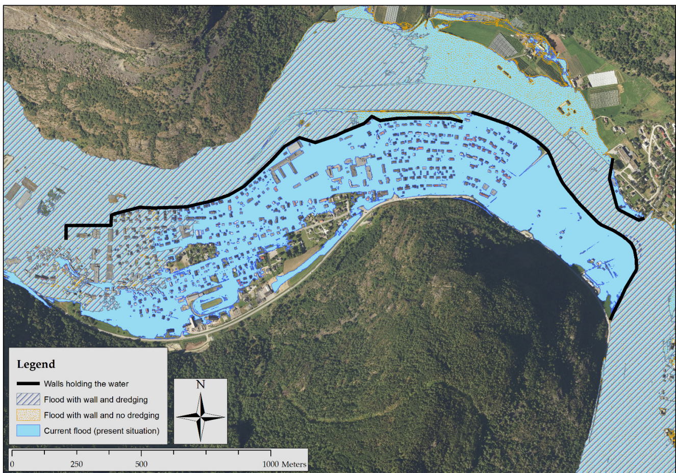
Figure 5. Flooded area at current situation (blue), with wall and no dredging (dotted) and with wall and dredging (stripes) with discharge 920 m^3/s .
