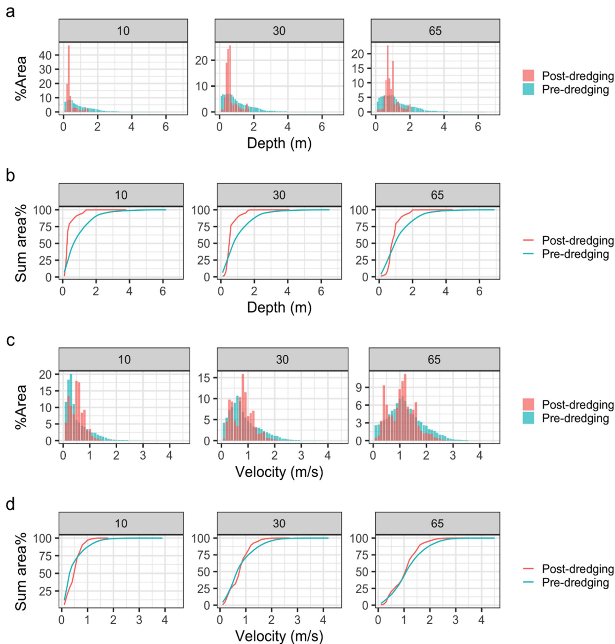
Figure 7. Histogram in % (a,c) and accumulated area in % (b,d) for depth and velocities at low, average, and high flows (10, 30, and 65 m 3 /s).
