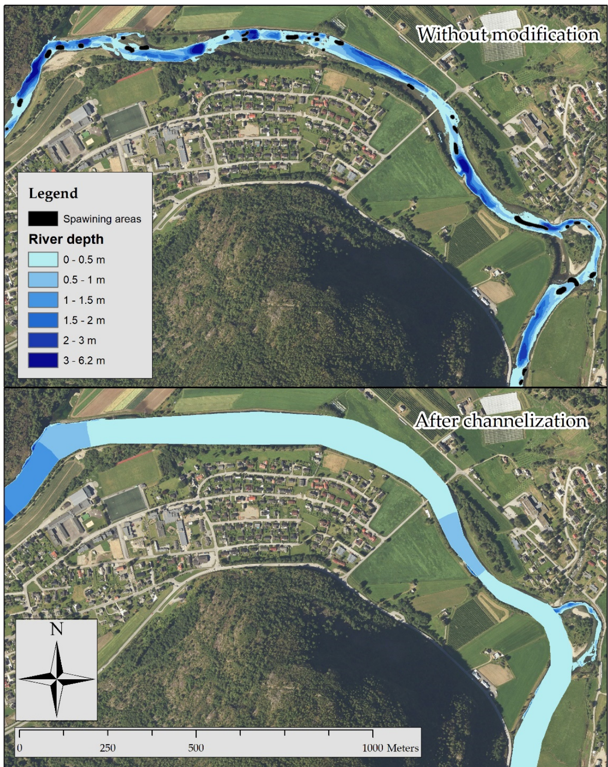
Figure 8. Map of river depths without river modification (top) and after channelization (bottom) at 10 m 3 /s.
