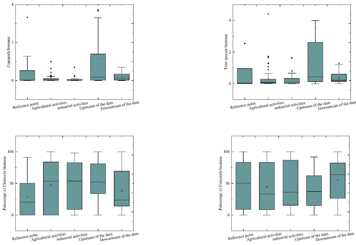
Figure S1: Multiple metrics in different areas of the Wanan River basin, China.
