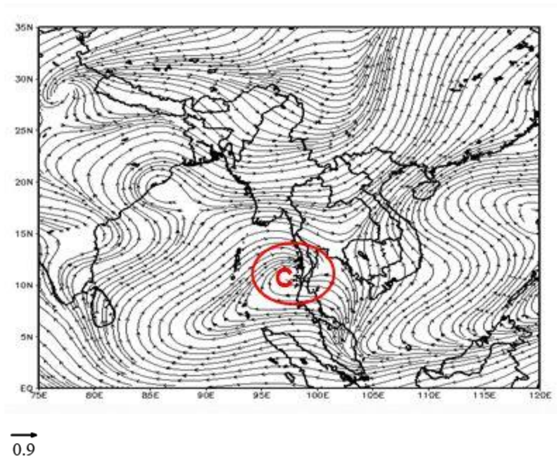
Figure S2. Difference stream fields of wet period (1962–1967, 1998, 2003–2004) minus dry period (1978–1986, 1988–1990) at 850 hPa in summer.
