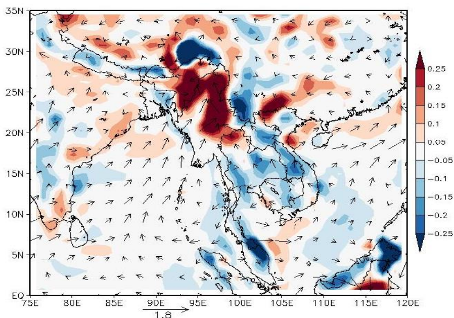
Figure S1. Difference fields of wet period (1962–1967, 1998, 2003–2004) minus dry period (1978–1986, 1988–1990) of moisture transport at 850 hPa ( \text{g kg}^{-1} \text{ms}^{-1} ) over Myanmar computed from ERA-interim dataset. Vector shows moisture transport, while the shaded regions specify convergence (positive) and divergence (negative) moisture fluxes convergence.
