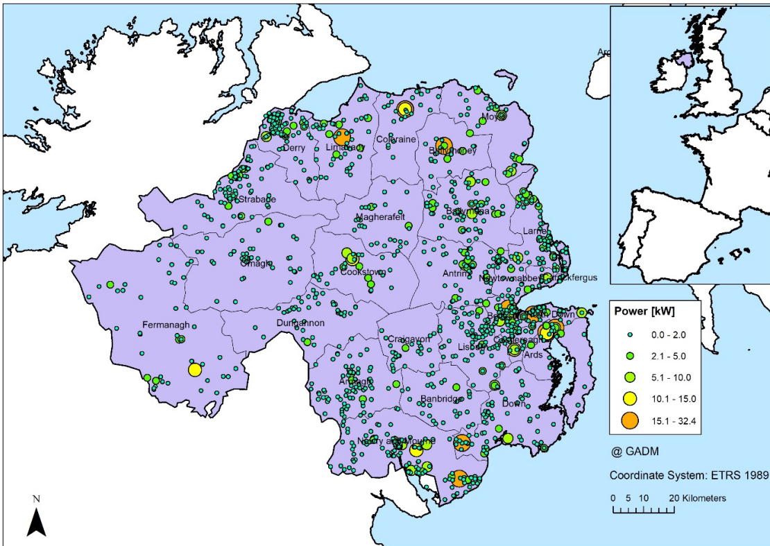
Figure S1. MHP energy recovery potential of sites identified in Ireland for the drinking water sector.
