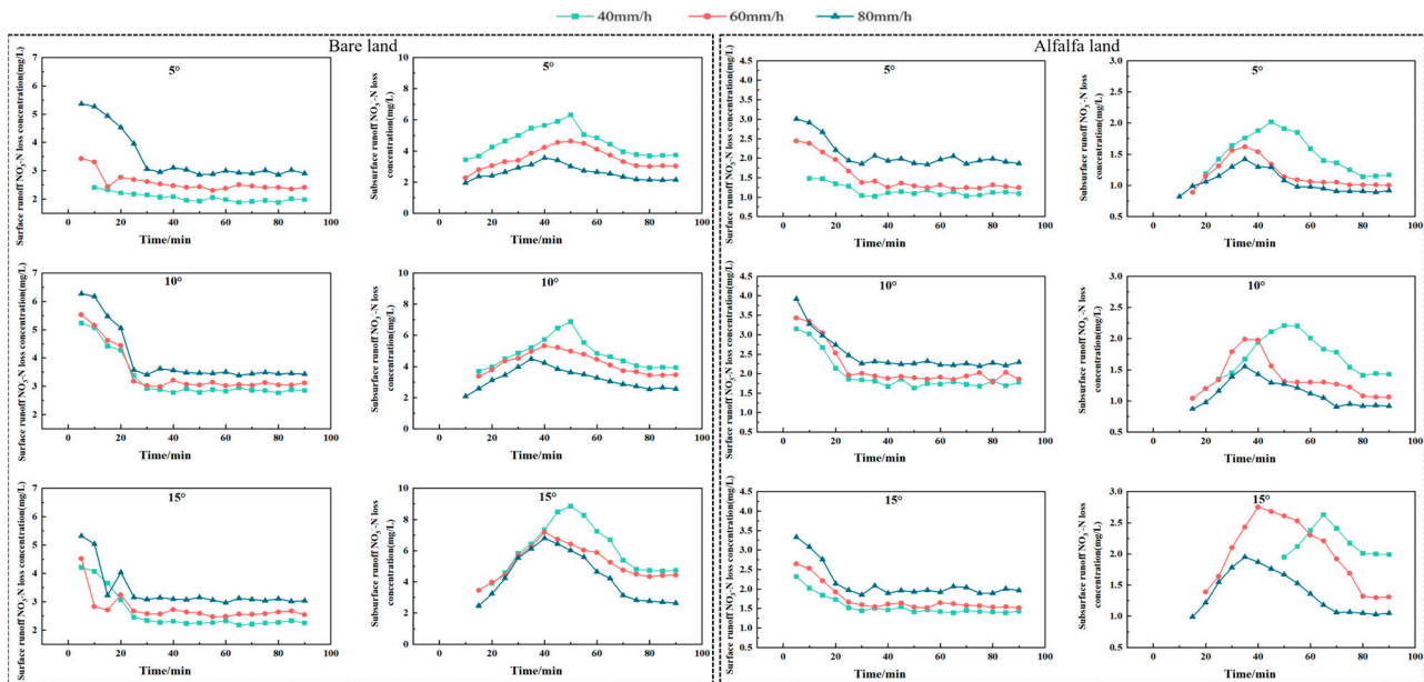
Figure 3. Dynamic variation curves of \text{NO}_3^- -N loss (mg/L) in surface and subsurface runoff for different rainfall intensities and slopes in bare and alfalfa-covered soils.
