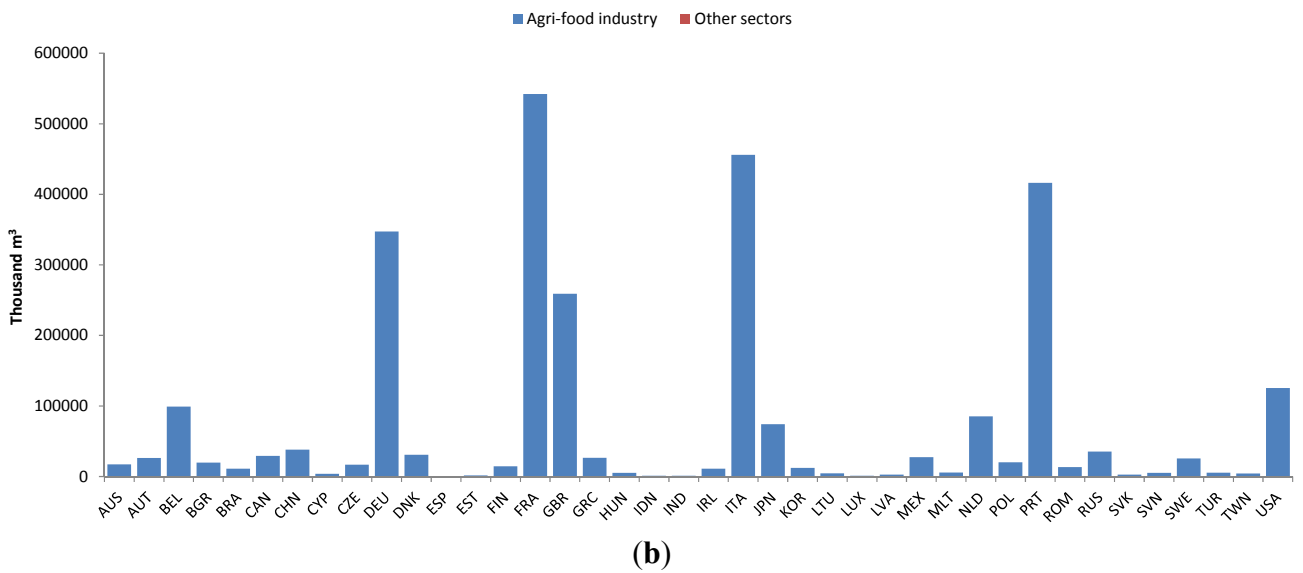
Figure S2. Grey virtual water exports of the agri-food sector by country and sector in 1995 (a) and 2009 (b), thousand m 3 .
