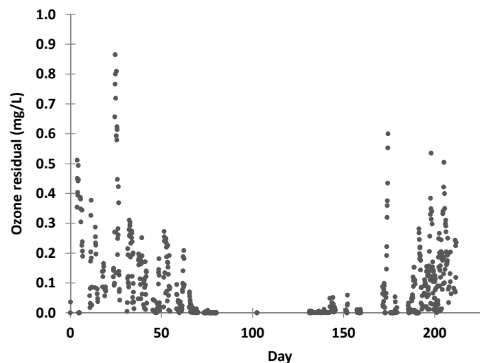
Figure 3. Ozone residual at the ozone contact tank outlet.
