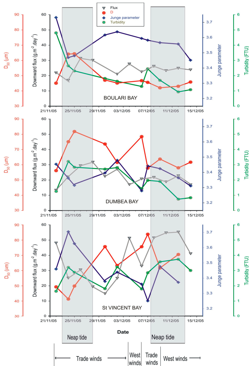
Figure 3. Median diameter ( D_{50} ), Jungge parameter ( s ), flux and turbidity for Boulari, Dumbéa and St Vincent bays over the study period (21 November to 14 December 2005), 3 m above the seabed.
