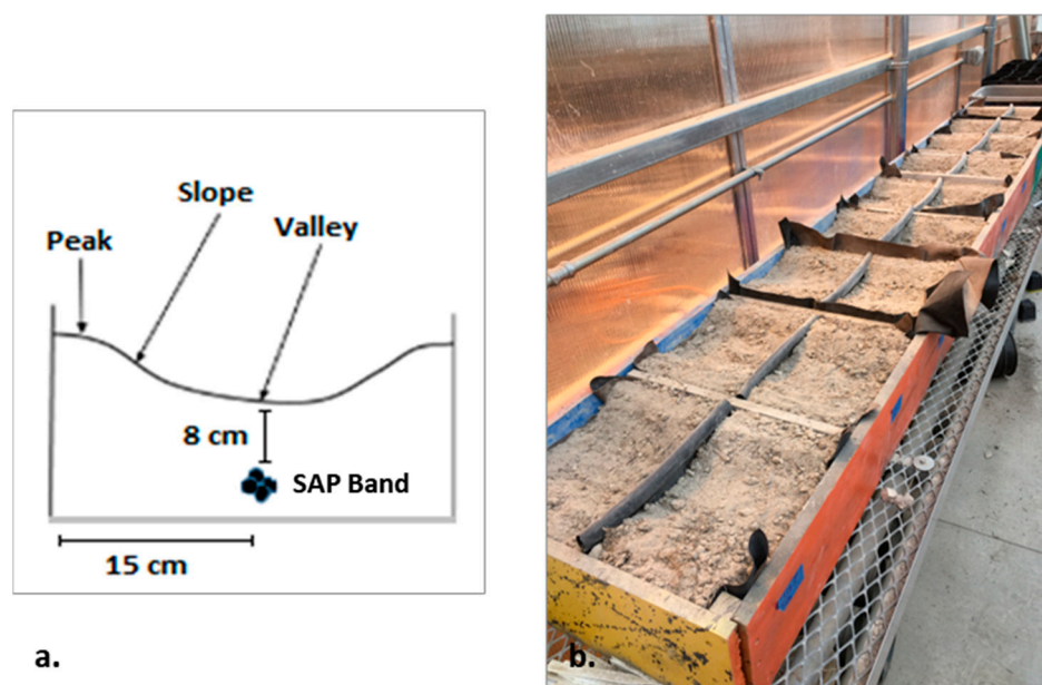
Figure 1. Frontal cross section diagram (a) of a grow box unit (b) containing soil with a superabsorbent polymer (SAP) band 8 cm below the soil surface of the furrow valley.
