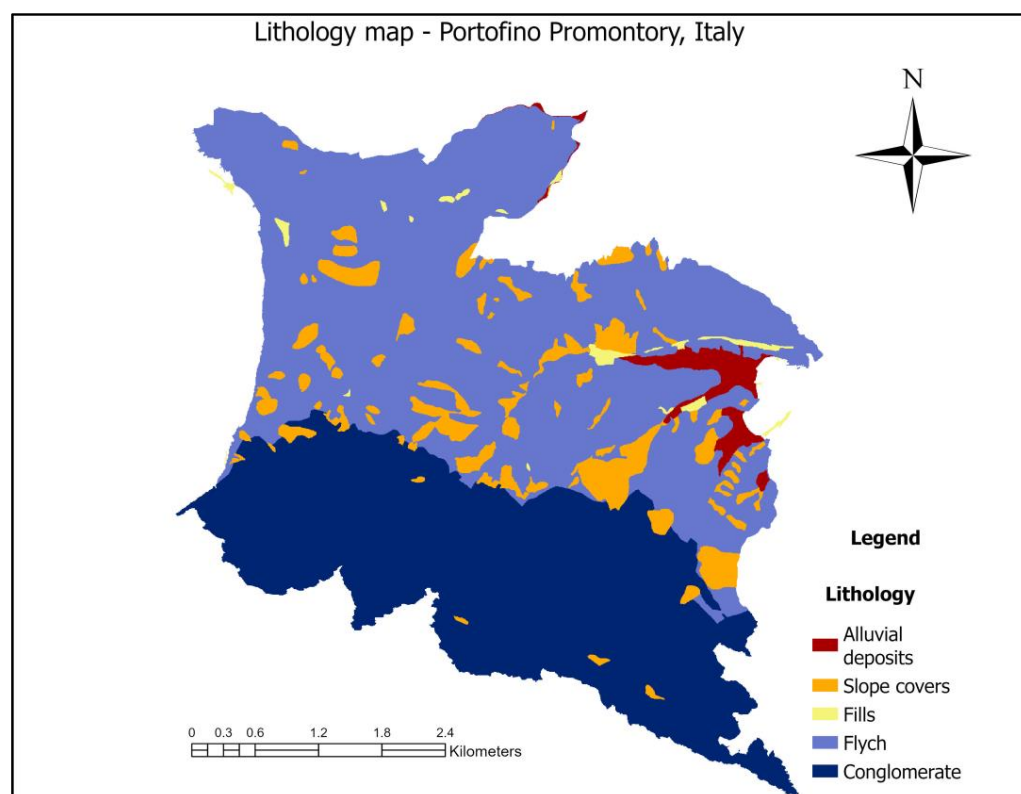
Figure 2. Lithology map of Portofino Natural Park.
