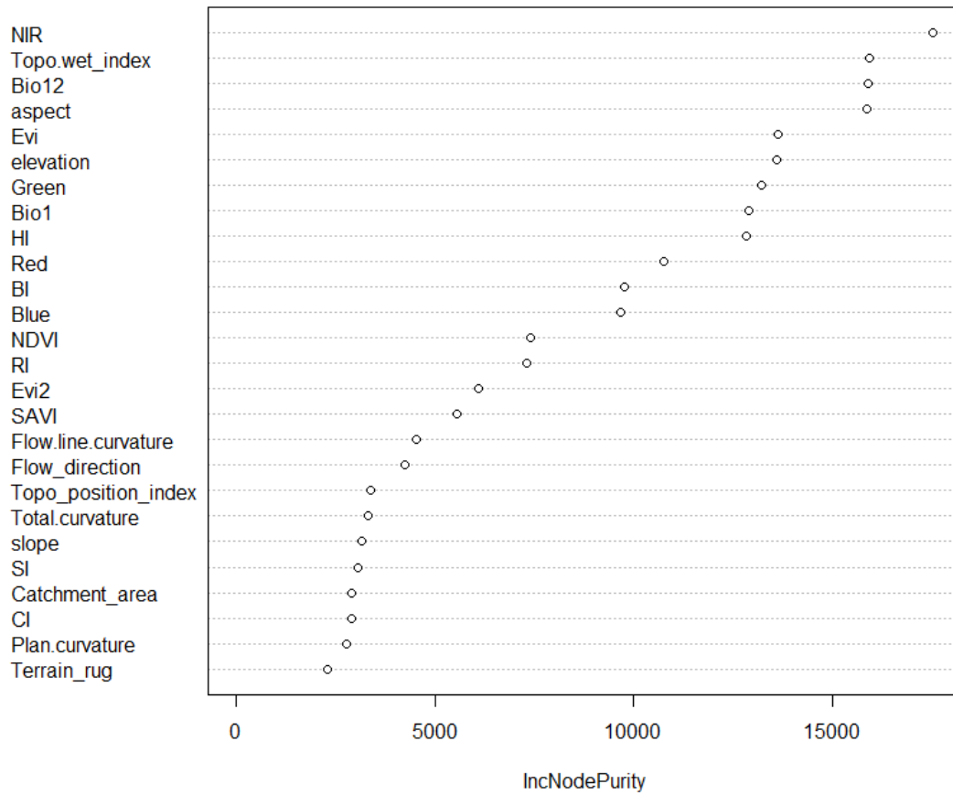
Figure SI1. Variable importance derived from RF models for carbon stock (NIR, Green, Red, Blue represent the near infra-red, green, red and blue bands from the S-2 image; Topo.wet_index: topographic wetness index; Bio12: precipitation; Bio1: temperature, HI: hue index; BI: brightness index; RI: redness index; SI: saturation index; CI: coloration index; Topo_position_index: topographic position index; Terrain_rug: terrain ruggedness)
