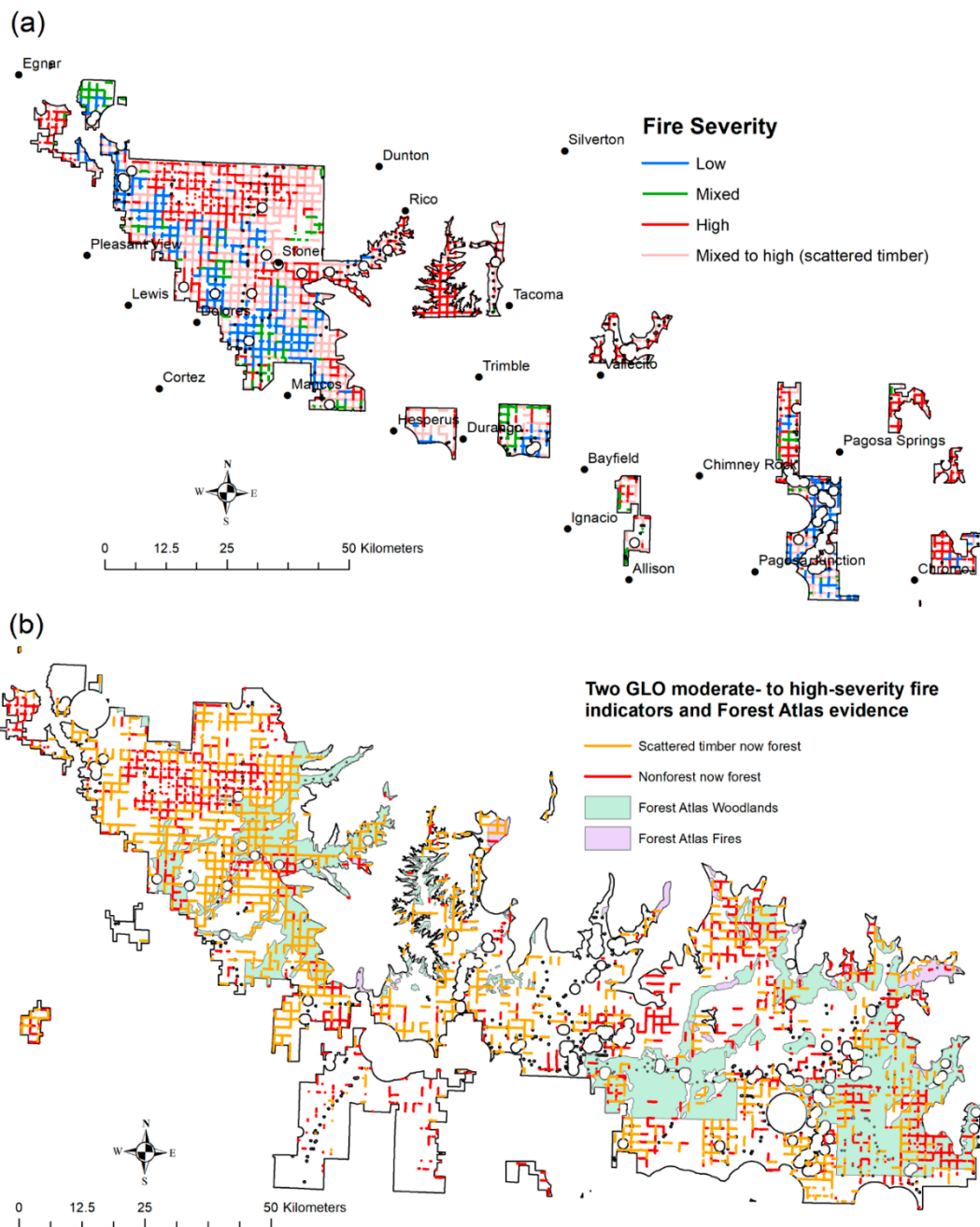
Figure 10. Reconstructed historical fire severity: (a) Based on section-corner and section-line data, and (b) based on only section-line data.
