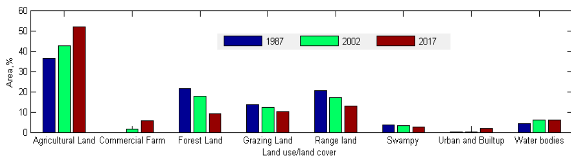
Figure 2. Land use/land cover distribution.
