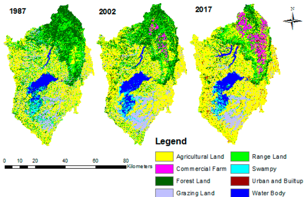
Figure 3. LULC map of Finchaa catchment in 1987, 2002, and 2017.
