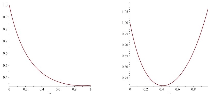
(a) g(t) = t
