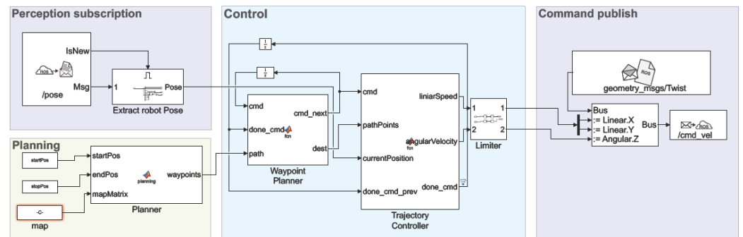
Figure 6. ROS application nodes implemented in Matlab.
