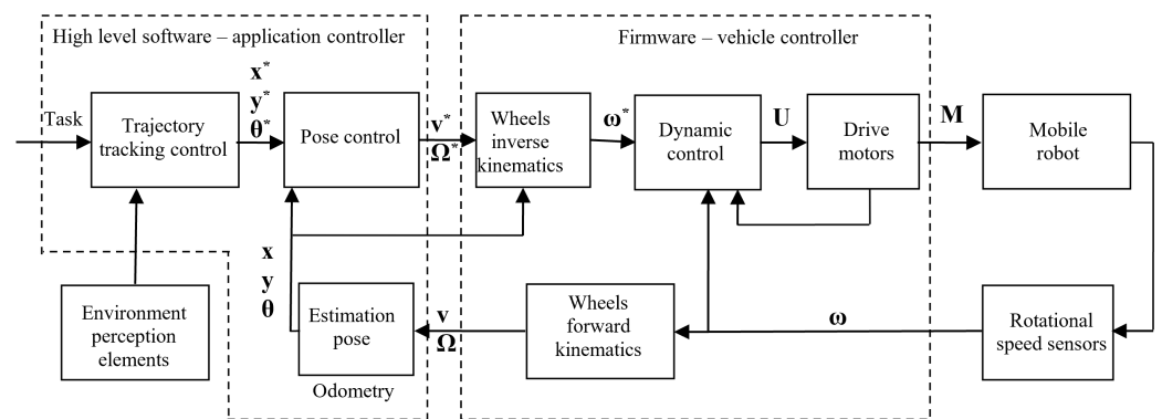
Figure 2. Controller structure of the mobile robot.
