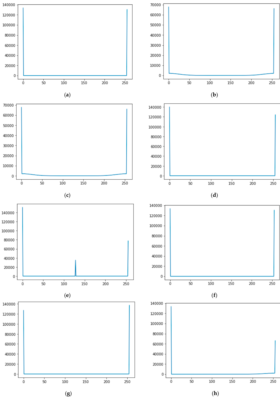
Figure 14. Histogram analysis of normal and noisy quick response (QR) code images where the x-axis represents the pixel number and the y-axis shows the value. (a) Normal QR codes; (b) Gaussian noisy QR codes; (c) Localvar noisy QR codes; (d) Pepper noisy QR codes; (e) Poisson; (f) Salt and pepper noisy QR codes; (g) Salt noisy QR codes and (h) Speckle noisy QR codes.
