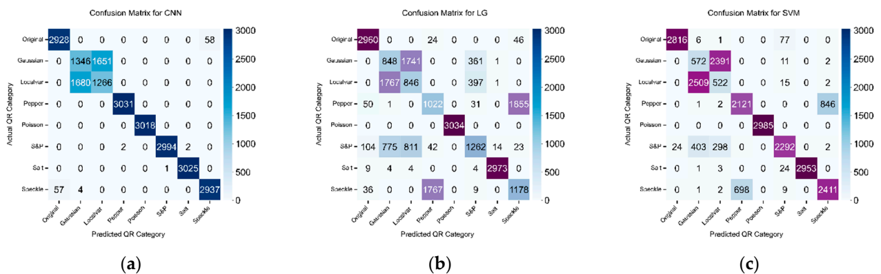
Figure 9. The confusion matrices for proposed classifiers when trained without external feature extraction technique to classify original quick response (QR) code and 7 different types of noisy QR code images. (a) convolutional neural network (CNN); (b) logistic regression (LG); and (c) support vector machine (SVM).
