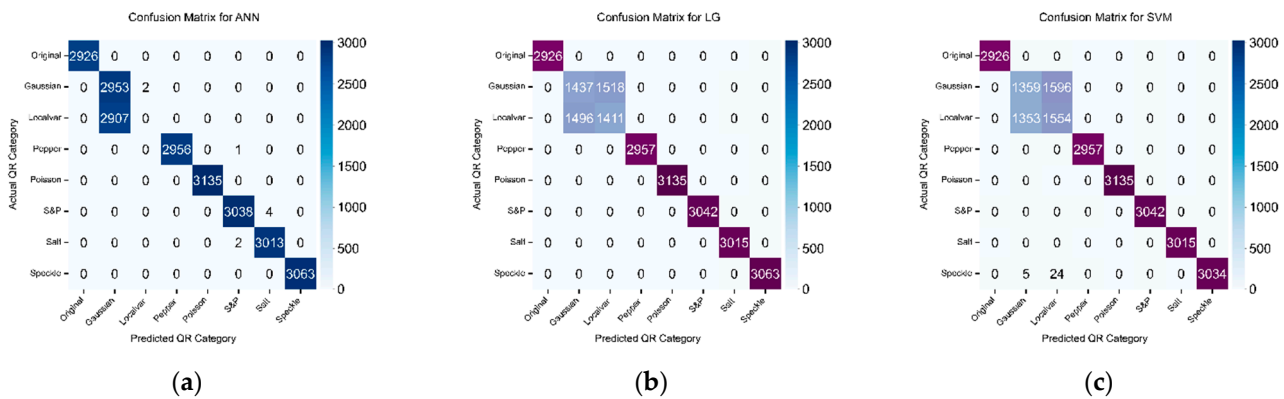
Figure 16. The confusion matrices for proposed classifiers when trained with features extraction through histogram density feature extraction technique to classify original quick response (QR) code and 7 different types of noisy QR code images. (a) artificial neural network (ANN); (b) logistic regression (LG); and (c) support vector machine (SVM).
