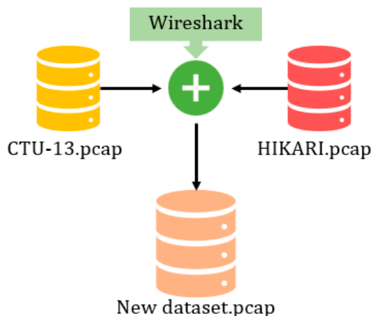
Figure 2. Data Construction.
