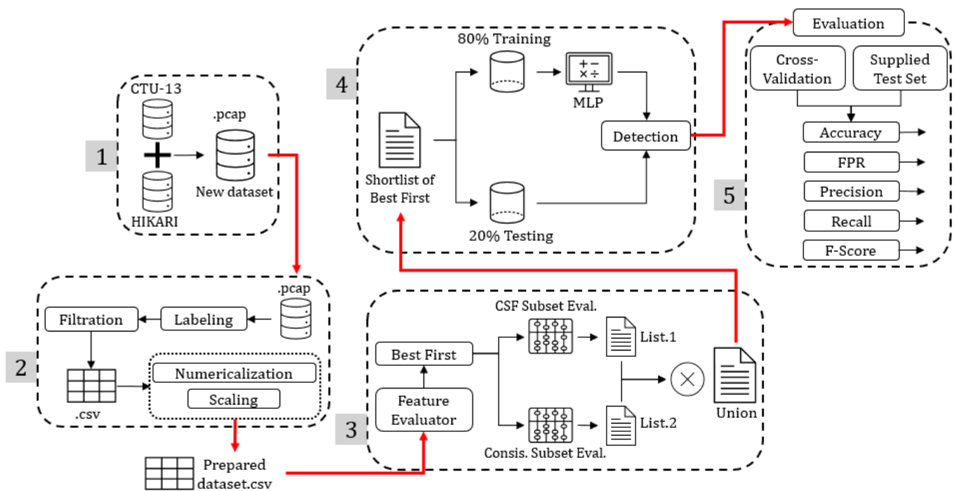
Figure 7. The roadmap of PeerAmbush.
