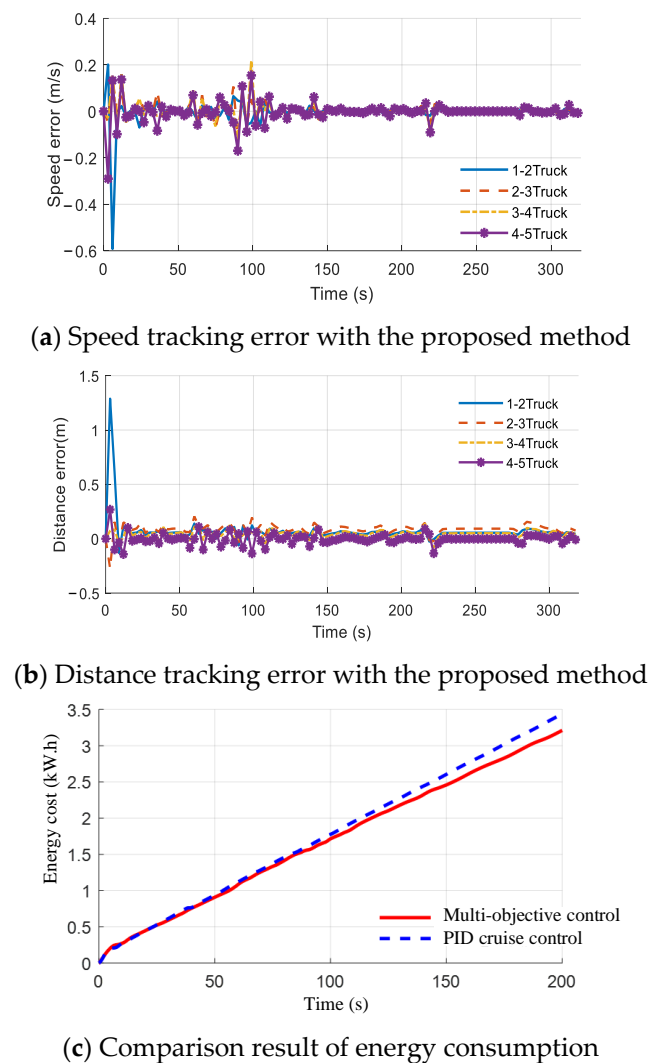
Figure 8. Test results of the heterogeneous platoon driving on the actual highway with varying slopes.
