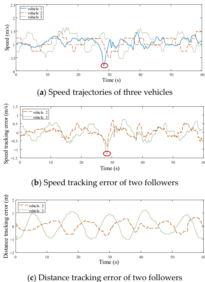
Figure 12. Results of the real-road experiment.
