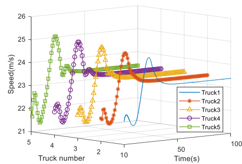
(a) Speed curve of each vehicle with the proposed method
