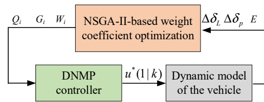
Figure 4. Control block diagram with the NSGA-II-based weight coefficient optimization method.
