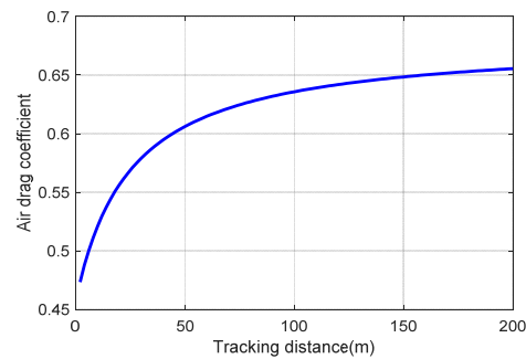
Figure 3. Relationship between air drag coefficient and the spacing.
