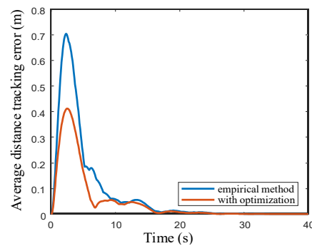
(b) Average distance tracking error of the platoon
