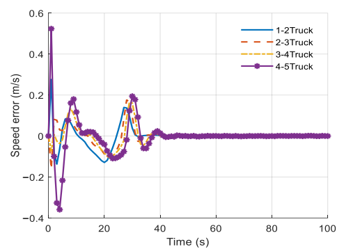
(b) Speed tracking error with the proposed method
