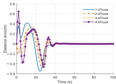
(c) Distance tracking error with the proposed method
