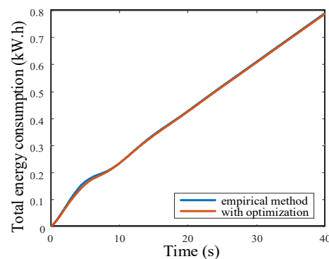
(c) Total energy consumption of the platoon
