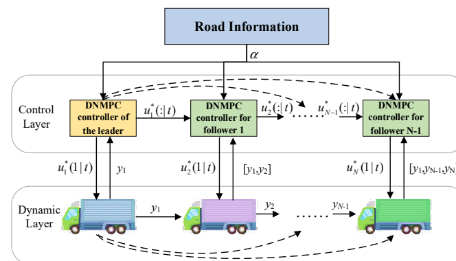
Figure 1. Architecture of the multi-objective control system of a heterogeneous platoon.
