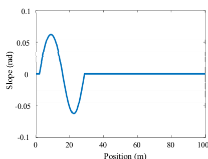
Figure 5. Slope curve of the designed road.
