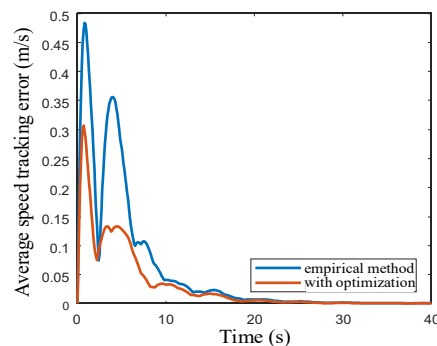
(a) Average speed tracking error of the platoon
