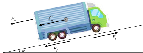
Figure 2. Force analysis of a vehicle on the ramp.
