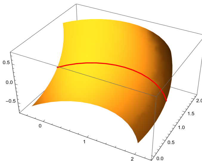
Figure 1. The curve \varphi(s) on M(s, v) .
