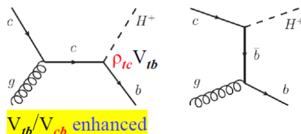
Figure 7. The |V_{tb}/V_{cb}| enhancement of cg \rightarrow bH^+ process w.r.t. 2HDM-II. H^+ \rightarrow t\bar{b} decay receives the same CKM factor V_{tb} multiplying \rho_{tt} [37].
