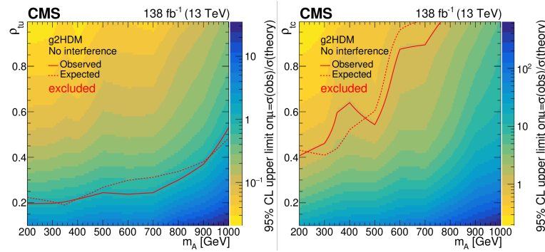
Figure 5. Observed 95% CL upper limit on signal strength vs m_A and \rho_{tu} (left) and \rho_{tc} (right) for G2HDM without A-H interference, for the combination of e^\pm e^\pm , \mu^\pm \mu^\pm , and e^\pm \mu^\pm categories. The color axis represents the observed upper limit on the signal strength. Expected (dashed) and observed (solid) exclusion contours are also shown (taken from Figure 6 of Ref. [39]).
