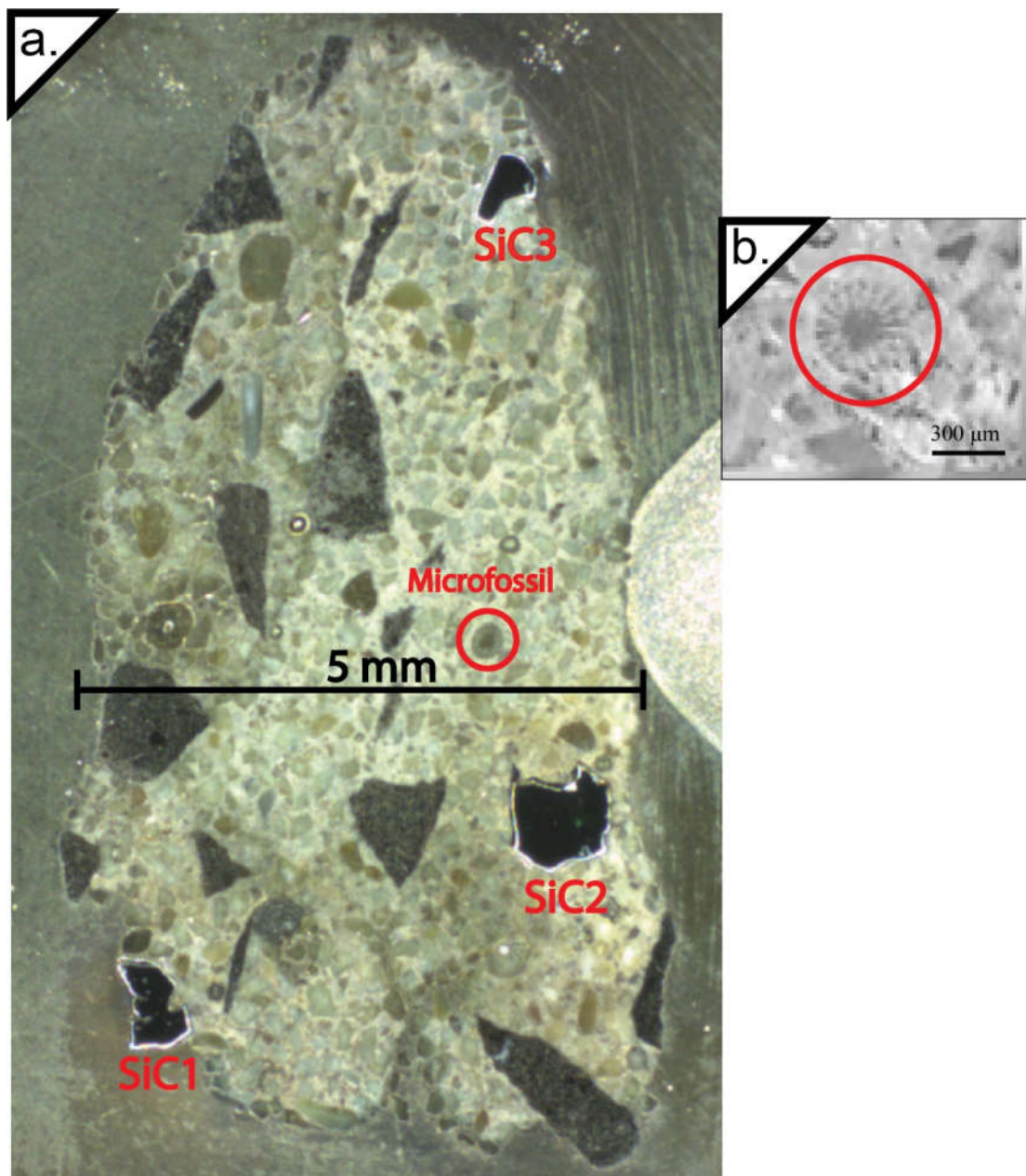
Figure S1. (a). Optical microscope image of the tuffite sample containing 3 SiC crystals. The red outline indicates the location of the microfossil/microfauna. (b). Microfossil/microfauna as seen at larger magnification.
