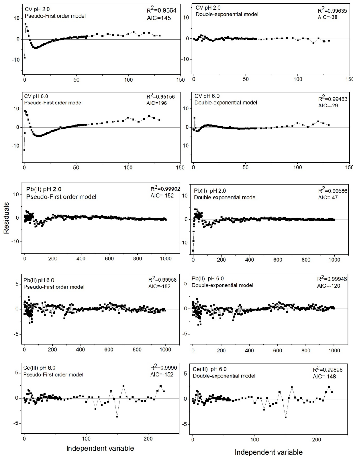
Figure S2. Residuals plot for the kinetic profiles reported in Figure 6 fitted by Pseudo-first order and Double Exponential Models.
