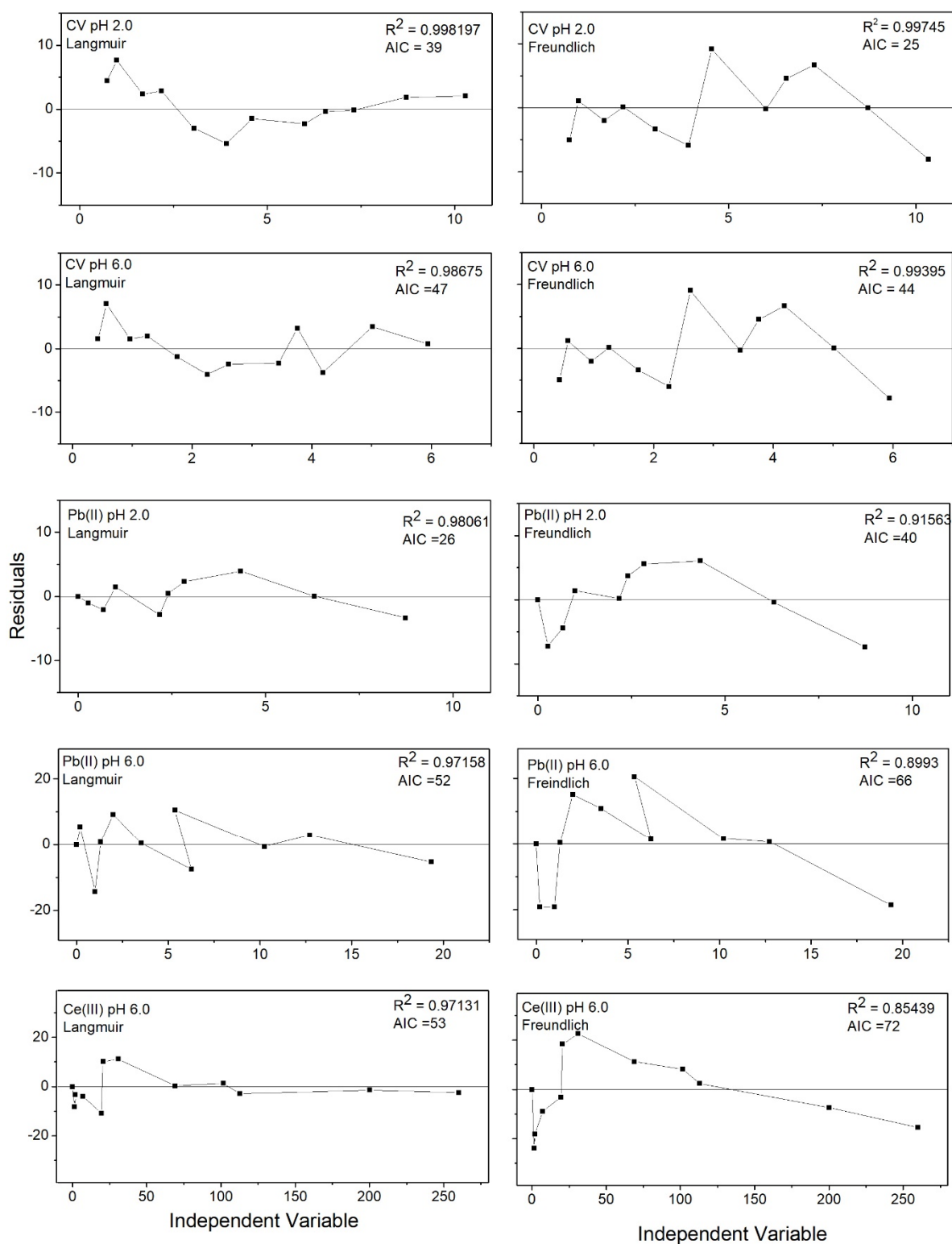
Figure S1. Residuals plot for the adsorption isotherms reported in Figure 4, fitted by using the Langmuir and the Freundlich models.
