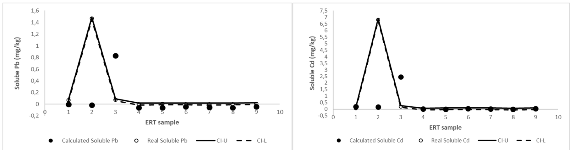
Figure S1. Relationship between the real parameter and the calculated parameter using the calibrated model obtained for each soil property and metal (CIU.: upper limit of the confidence interval; CI-L.: lower limit of the confidence level; Bioav.: bioavailable).
