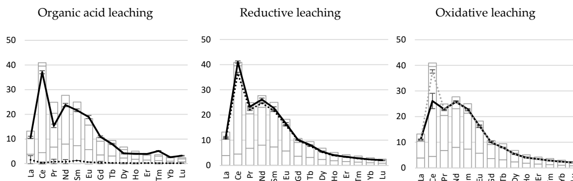
Figure 5. Recovery (%) of individual REE from low-Ca bauxite for each of the leaching techniques tested. Solid lines represent inoculated tests and dotted lines are uninoculated controls. Error bars are plus or minus one standard deviation of triplicate experiments. Bar charts show sequential extraction data, as in Figure 4.
