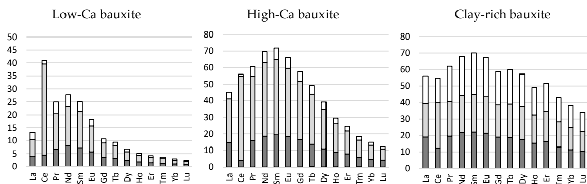
Figure 4. Recovery (%) of individual REE using sequential extraction. Leaching from step 1 exchangeable (magnesium chloride) is not visible; step 2, dark grey—acid soluble (acetic acid); step 3, pale grey—reducible (hydroxylamine hydrochloride); step 4, white—oxidisable (hydrogen peroxide).
