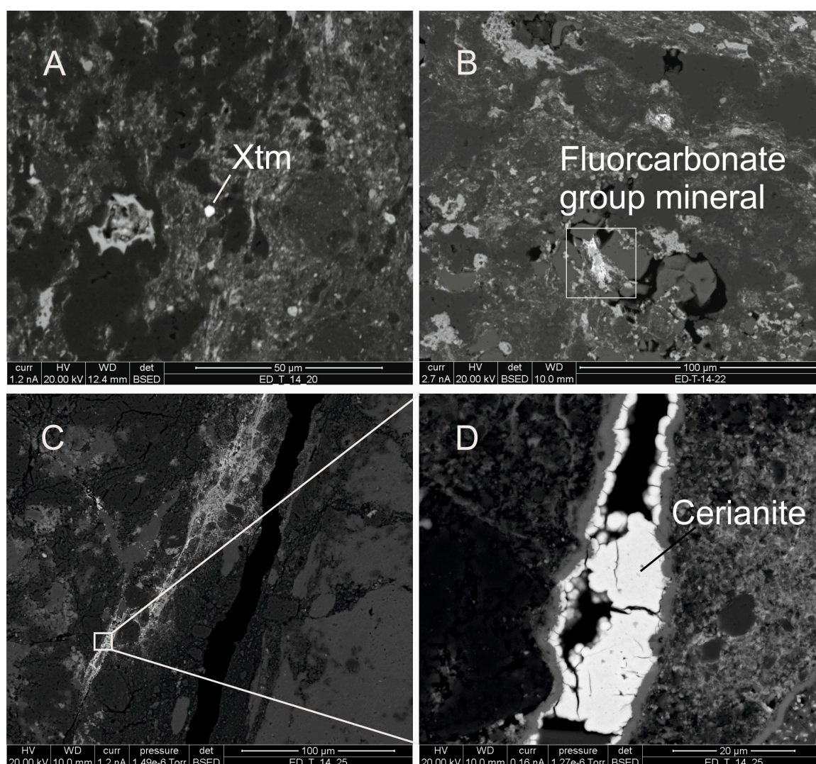
Figure 3. (A) Low-Ca bauxite—xenotime (Xtm) in the matrix; (B) High-Ca bauxite—interstitial fluorcarbonate; (C) Clay-rich bauxite—framboidal cerianite infill along fractures; (D) Clay-rich bauxite—framboidal cerianite in fractures.
