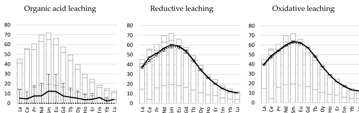
Figure 6. Recovery (%) of individual REE from high-Ca bauxite for each of the leaching techniques tested. Solid lines represent inoculated tests and dotted lines are uninoculated controls. Error bars are plus or minus one standard deviation of triplicate experiments. Bar charts show sequential extraction data, as in Figure 4.
