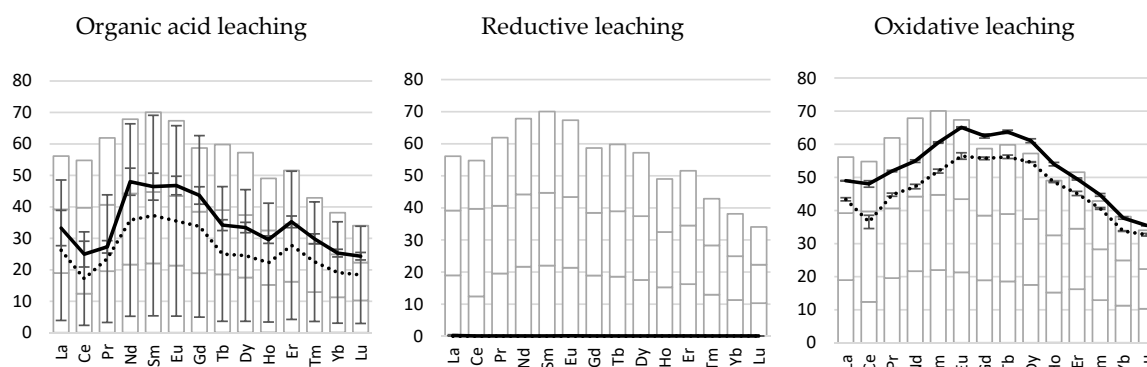
Figure 7. Recovery (%) of individual REE from clay-rich bauxite for each of the leaching techniques tested. Solid lines represent inoculated tests and dotted lines are uninoculated controls. Error bars are plus or minus one standard deviation of triplicate experiments. Bar charts shows sequential extraction data, as in Figure 4.
