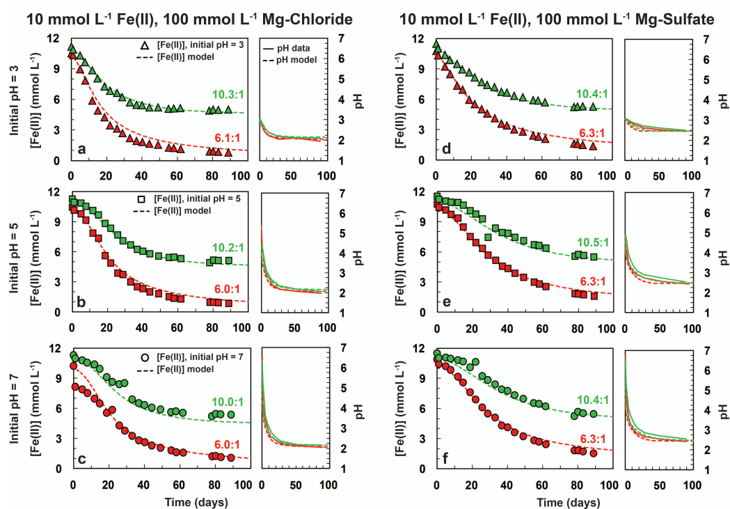
Figure 1. The dissolved Fe(II) concentration and pH versus time in systems containing approximately 10 mmol L -1 Fe(II) with 1.67 ( [\text{Fe(II)}]/[\text{ClO}_3^-] \approx 6 ) mmol L -1 and 1 mmol L -1 ( \approx 10 ) ClO 3 - in 10 -1 mol L -1 MgCl 2 at initial (a) pH 3, (b) pH 5, and (c) pH 7, and in 10 -1 mol L -1 MgSO 4 fluids at initial (d) pH 3, (e) pH 5, and (f) pH 7 at 24 °C. The ratios written alongside the curves represent the initial molar ratio between [Fe(II)] and [ClO 3 - ].
