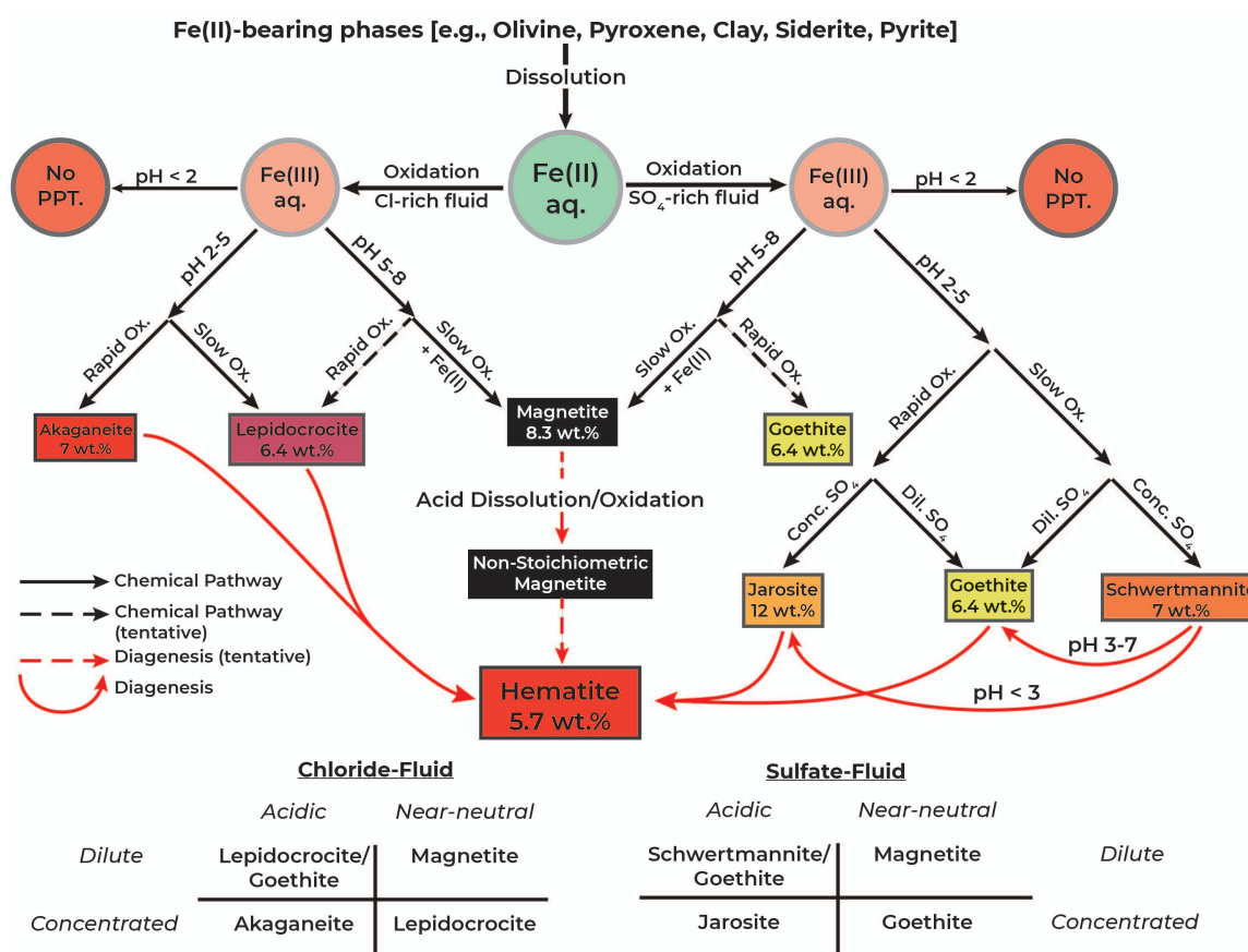
Figure 3. (Top) Schematic of possible iron oxidation pathways on Mars. Mineral products of iron oxidation determined by the fluid type, solution pH, and oxidation rate. The wt.% in each mineral box represents the amount of Fe(III)-bearing mineral that can be produced by the oxidation of Fe(II) by 1 wt.% chlorate. (Below) Fourfold diagram depicting the dominant mineral product as a function of fluid concentration and solution pH.
