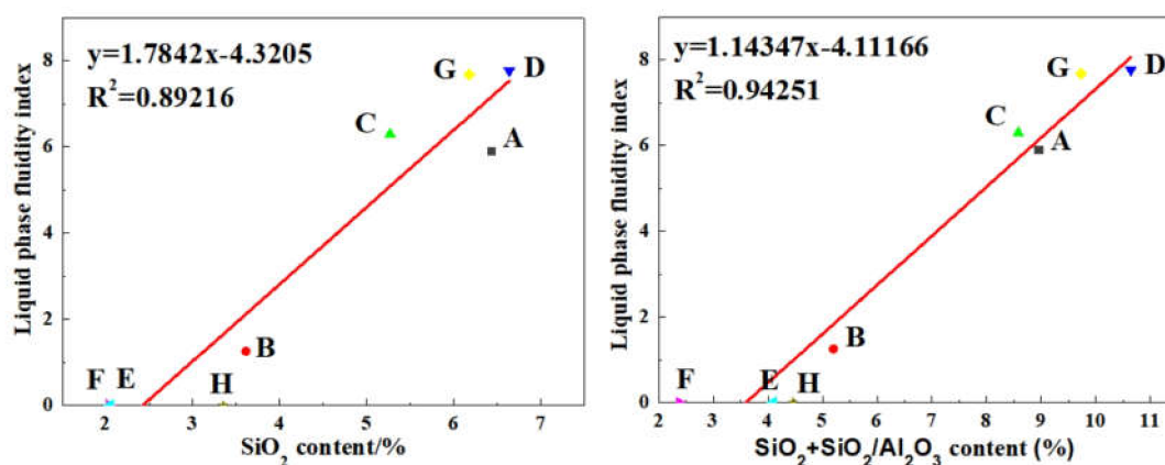
Figure A3. Correlation between chemical compositions and liquid phase fluidity of iron ores.
