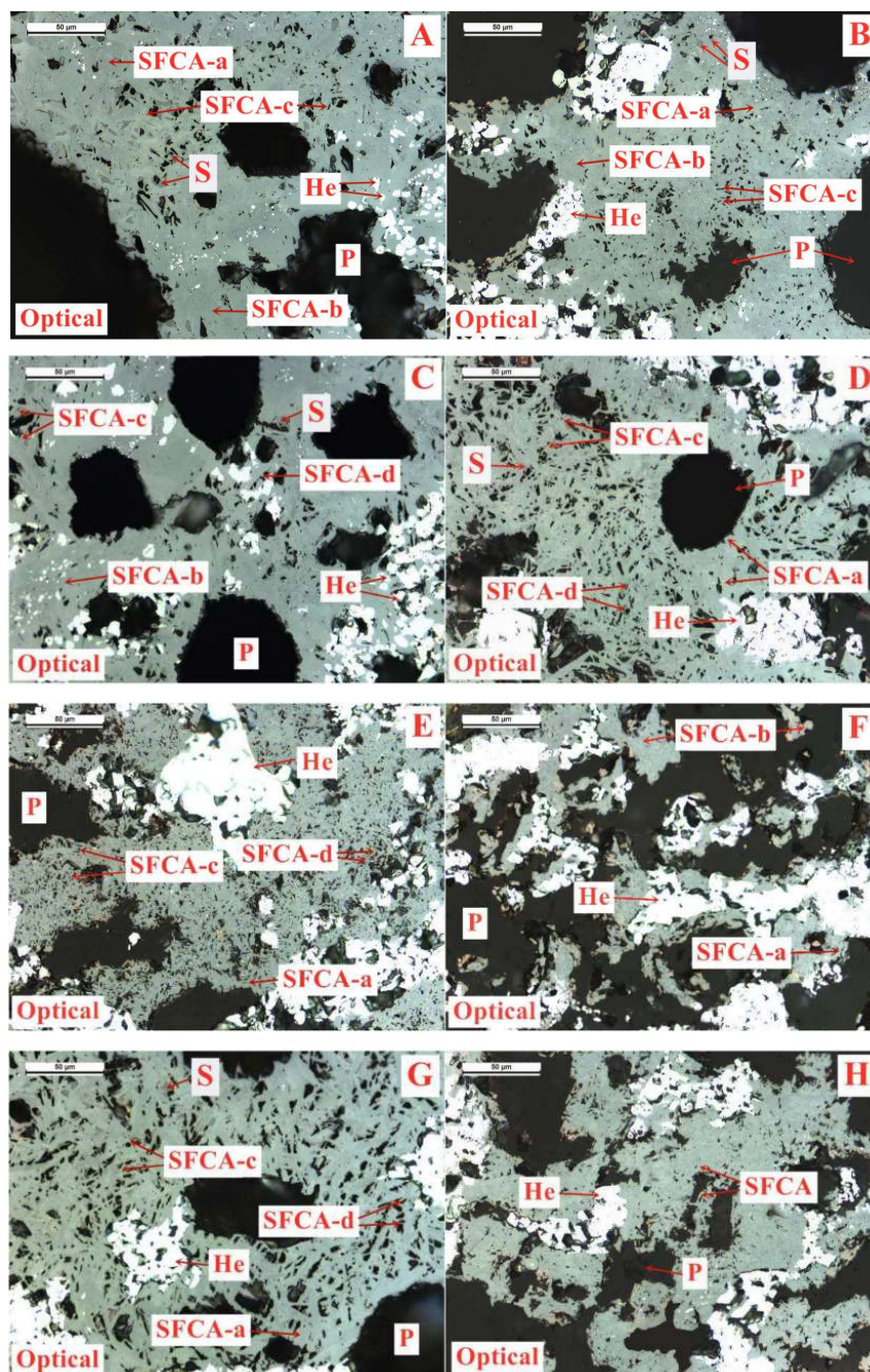
Figure 7. Characteristics of the bonding matrix in sinter tablets of various types of iron ores ((A–H) represent the optical photographs of iron ores A–H respectively; He: Hematite; S: Silicate; SFCA-a-Tabular: SFCA; SFCA-b-Lamellar: SFCA; SFCA-c-Dendritic: SFCA; SFCA-d-Acicular: SFCA; P: Pores).
