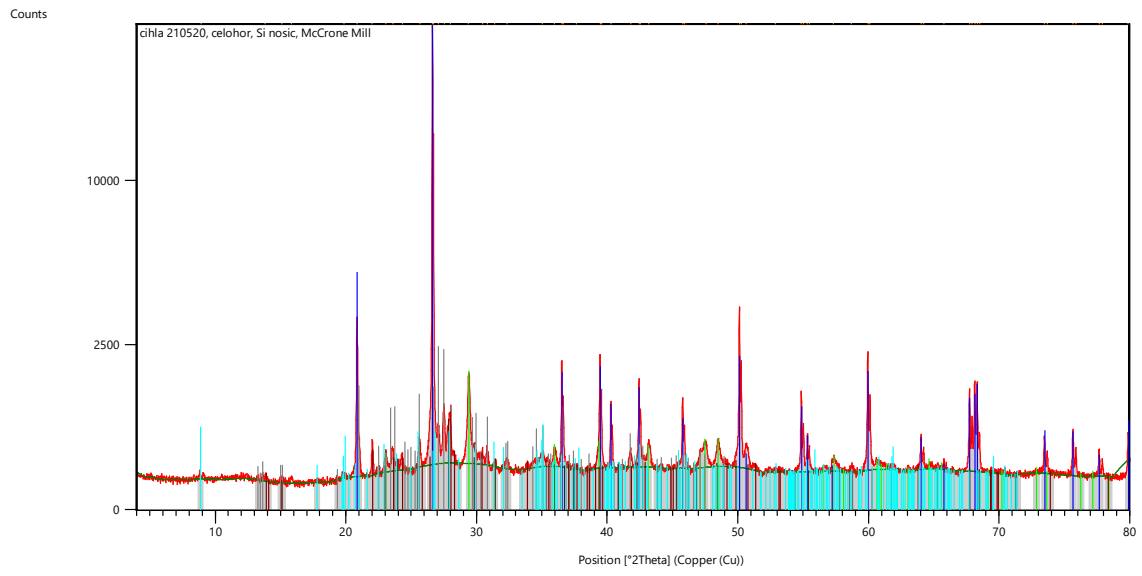
Figure S5. Outdoor sample after 8 years.
