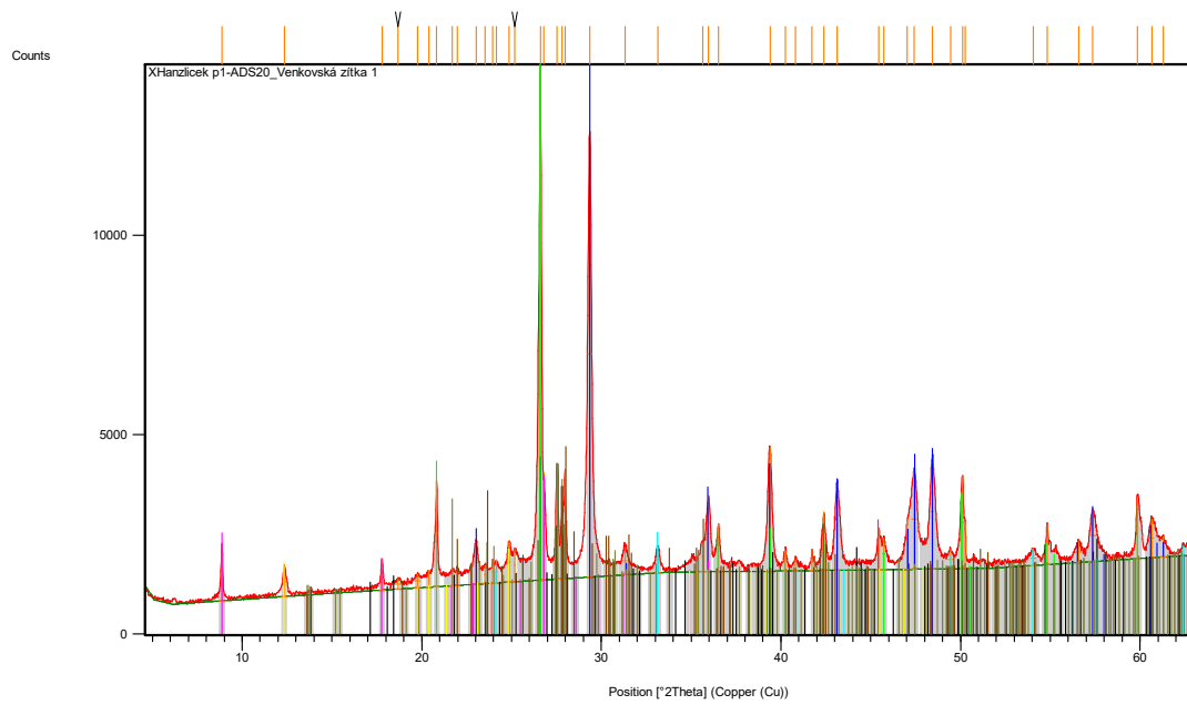
Figure S4. Outdoor sample after 2 years.
