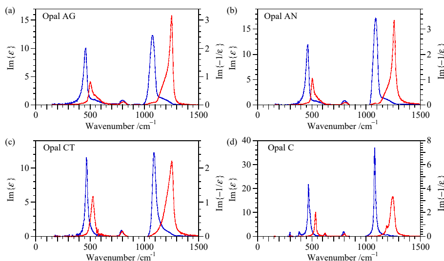
Figure 7. \text{Im}\{\varepsilon\} (blue) and \text{Im}\{-1/\varepsilon\} (red) spectra derived from a Kramers-Kronig transform of polished slabs showing TO and LO components, respectively. Samples are (a) opal-AG (CP-2 from Coober Pedy, South Australia, Australia), (b) opal-AN (MS-1 from mount Squaretop, Queensland, Australia), (c) opal-CT (G9942 from Angaston, South Australia, Australia) and (d) opal-C (T1664 from Guanajuato, Mexico). Note that the \text{Im}\{-1/\varepsilon\} spectrum is displayed 5× enhanced compared to the \text{Im}\{\varepsilon\} spectrum. \text{Im}\{\varepsilon\} values are given on the left axis and \text{Im}\{-1/\varepsilon\} values are displayed on the right axis.
