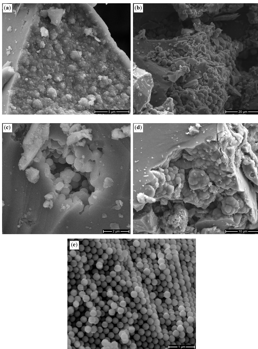
Figure 15. SEM images of selected zones of “opaline” silica samples and Gilson synthetic opal. (a) G21471 (geyserrite from Rotorua, New Zealand), (b) T1665 (geyserrite from Rotorua, New Zealand), (c) G NEW23 (Spanish menilite from Caldes de Malvella, La Selva, Catalonia, Spain), (d) G NEW01 (Spanish menilite from Caldes de Malvella, La Selva, Catalonia, Spain) and (e) Gilson synthetic opal. Note differences in scale.
