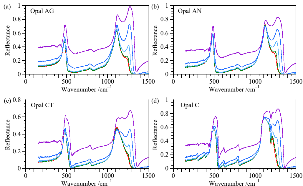
Figure 5. Specular reflectance spectra (unpolarised light) of polished thin segments of (a) opal-AG (CP-2 from Coober Pedy, South Australia, Australia), (b) opal-AN (MS-1 from Mount Sqauretop, Queensland, Australia), (c) opal-CT (G9942 from Angaston, South Australia, Australia) and (d) opal-C (T1664 from Guanajuanto, Mexico) (red 15°, green 30°, light blue 45°, blue, 60° and violet 75°).
