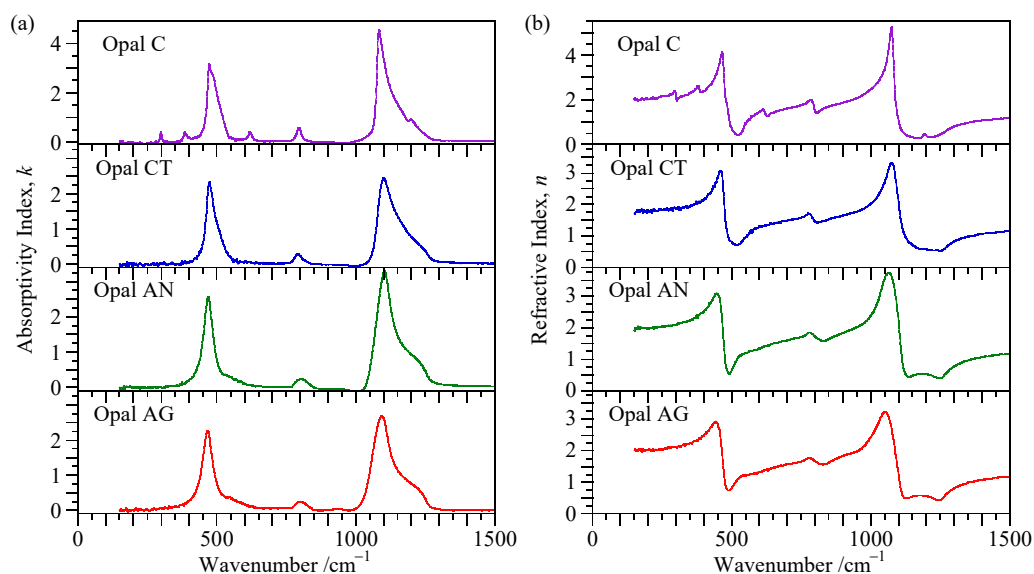
Figure 6. Kramers-Kronig-transformed spectra of polished slabs of (red) opal-AG (CP-2 from Coober Pedy, South Australia, Australia), (green) opal-AN (MS-1 from Mount Sqauretop, Queensland, Australia), (blue) opal-CT (G9942 from Angaston, South Australia, Australia) and (violet) opal-C (T1664 from Guanajuanto, Mexico); (a) the absorptivity index, k , and (b) the refractive index, n .
