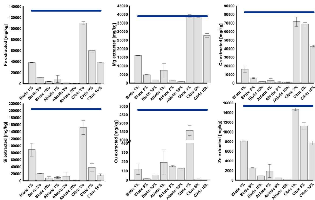
Figure 2. Two weeks long leaching of elements from glassy slag as a function of pulp density.
