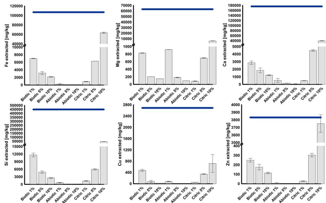
Figure 1. Two weeks long leaching of elements from diopside-bearing slag as a function of pulp density.
