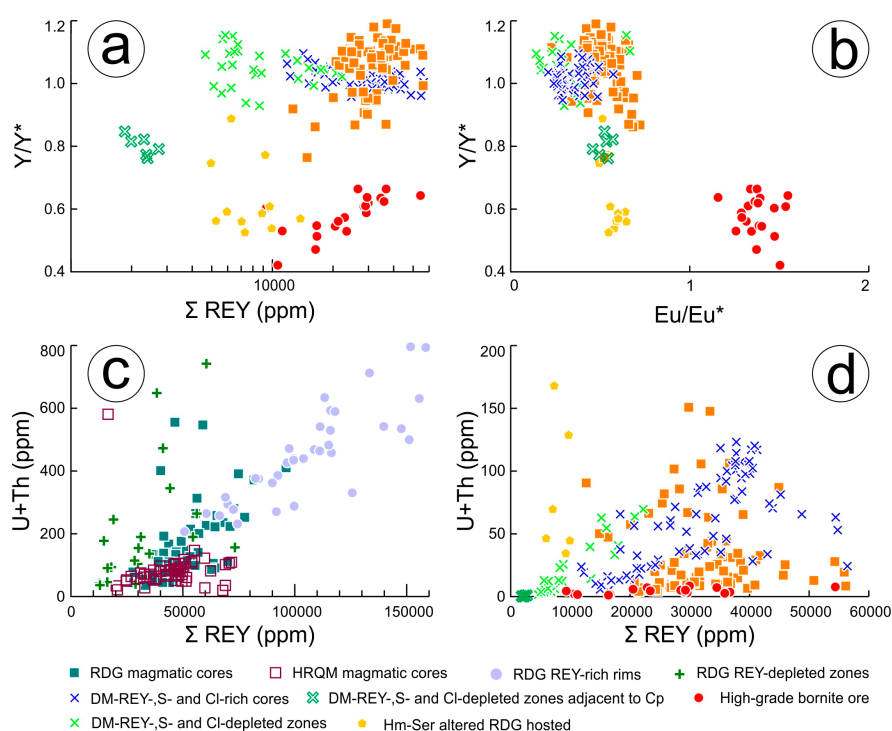
Figure 9. LA-ICP-MS plots of magmatic and hydrothermal apatite: (a) \Sigma\text{REY} (ppm) vs. ( Y/Y^* = Y_{\text{CN}}/[(D_{\text{YCN}} + H_{\text{OCN}})/2] ); (b) ( \text{Eu}/\text{Eu}^* = \text{Eu}_{\text{CN}}/[(\text{Sm}_{\text{CN}} + \text{Gd}_{\text{CN}})/2] ) vs. ( Y/Y^* = Y_{\text{CN}}/[(D_{\text{YCN}} + H_{\text{OCN}})/2] ); (a,b) The evolution from early magnetite associated to later hematite-sericite and ore-related apatite is emphasized by changes in \Sigma\text{REY} as well as Eu and Y anomalies; (c) \Sigma\text{REY} (ppm) vs. (U + Th) (ppm); (d) \Sigma\text{REY} (ppm) vs. (U + Th) (ppm). (c,d) U and Th concentrations are strongly tied to that of \Sigma\text{REY} , particularly in magmatic apatite and hydrothermal zones therein.
