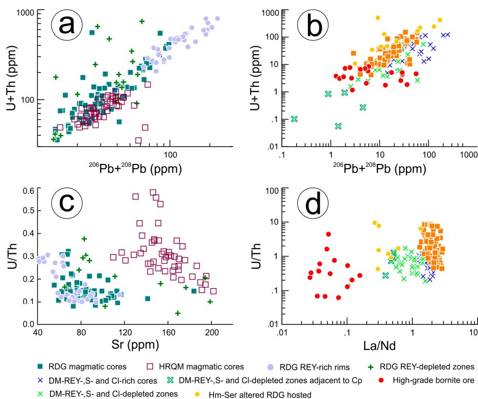
Figure 10. LA-ICP-MS plots of magmatic and hydrothermal apatite: (a) \log(^{206}\text{Pb} + ^{208}\text{Pb} \text{ ppm}) vs. (\text{U} + \text{Th}) (ppm); (b) \log(^{206}\text{Pb} + ^{208}\text{Pb} \text{ ppm}) vs. \log(\text{U} + \text{Th} \text{ ppm}) ; (a,b) U and Th concentrations exhibit a strong linear relationship with their lead daughter isotopes; (c) Sr (ppm) vs. (\text{U} + \text{Th}) (ppm); (d) La/Nd (ppm) vs. \log(\text{U} + \text{Th}) (ppm).
