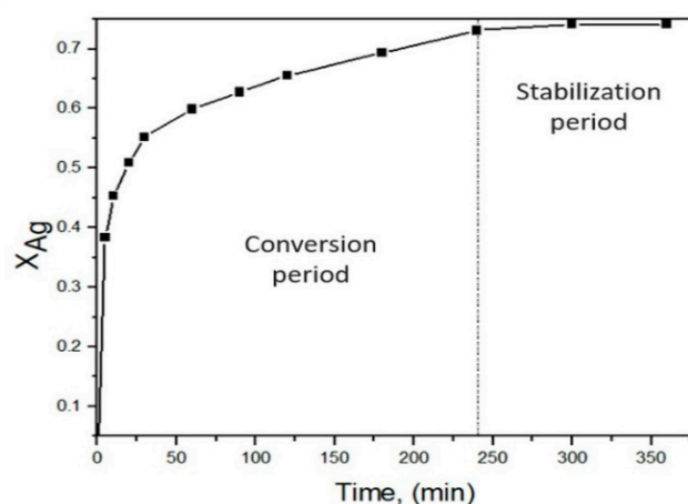
Figure 5. Dissolution curve of silver in the S_2O_3^{2-}-Cu^{2+} system ( V = 0.5 L, 40 g L^{-1} Mineral, PO_2 = 1 atm, pH = 10 , leaching time = 360 min, [S_2O_3^{2-}] = 0.16 mol L^{-1} , [Cu^{2+}] = 0.006 mol L^{-1} , 298 K ( 25 °C), RPM = 750 min^{-1} ).
