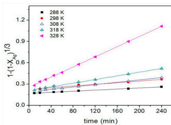
Figure 12. Assessment of the application of the chemical control model on the conversion values of Ag in function of time for the study of the temperature effect in the S_2O_3^{2-} - O_2 system, ( V = 0.5 L, 40 g·L ^{-1} Mineral, PO_2 = 1 atm, pH = 10 , leaching time = 240 min, [S_2O_3^{2-}] = 0.16 mol·L ^{-1} , [Cu^{2+}] = 0.006 mol·L ^{-1} , 298 K (25 °C), RPM = 750 min ^{-1} ).
