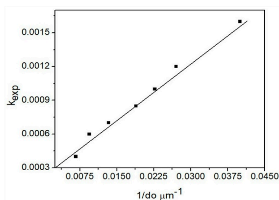
Figure 8. k_{\text{exp}} versus the inverse of particle diameter. ( V = 0.5 \text{ L} , 40 \text{ g}\cdot\text{L}^{-1} Mineral, \text{PO}_2 = 1 \text{ atm} , \text{pH} = 10 , leaching time = 240 min, [\text{S}_2\text{O}_3^{2-}] = 0.16 \text{ mol}\cdot\text{L}^{-1} , [\text{Cu}^{2+}] = 0.006 \text{ mol}\cdot\text{L}^{-1} , 298 K, \text{RPM} = 750 \text{ min}^{-1} ).
