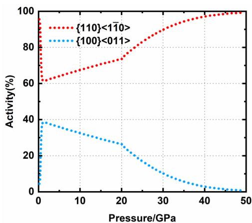
Figure 6. Activity of slip systems in EVPSC simulation. {110}<110> and {100}<011> slip systems are activated with a ratio of 70:30 and gradually reach 100:0 at ~50 GPa.
