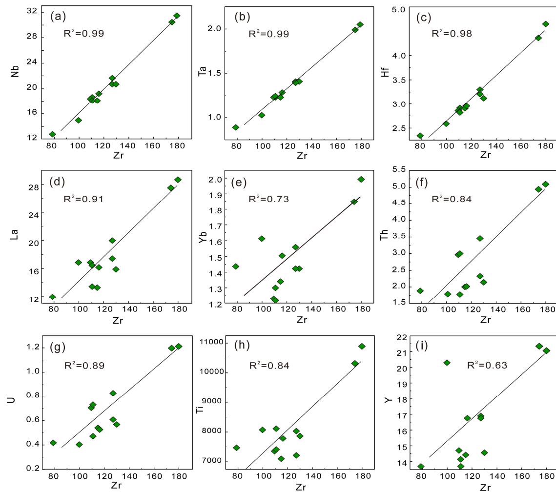
Figure S1. Elements versus Zr correlation diagrams for mafic intrusions in Jingxi, SW China.
