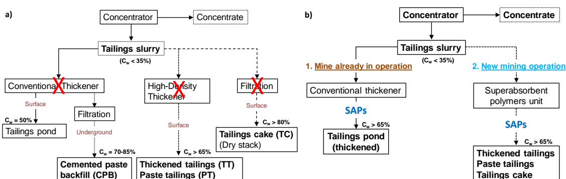
Figure 3. The use of SAPs to obtain densified tailings: (a) eliminating all conventional dewatering systems, (b) replacing all conventional dewatering system with SAPs, either for a mine already in operations or for new mine operations.
