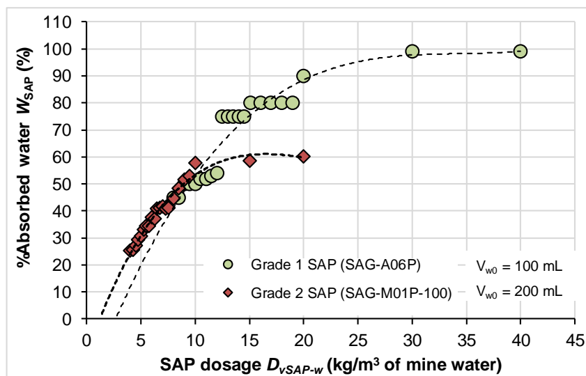
Figure 15. Mine A water absorption capacity of coarser SAP (grade 1 = SAG-A06P) and the finer SAP (grade 2 = SAG-M01P-100).
