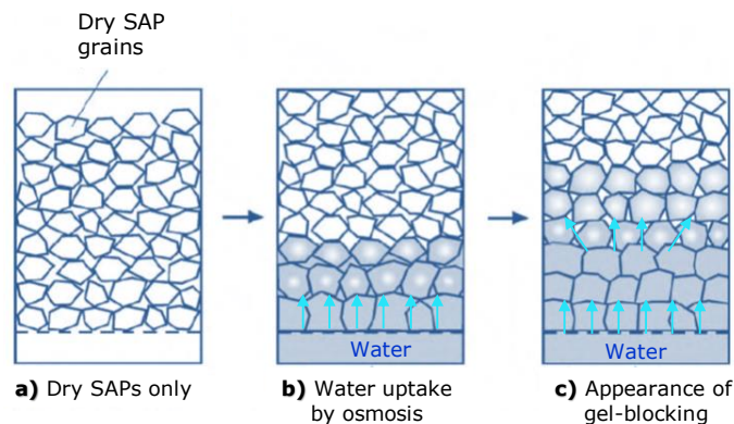
Figure 14. Schematic illustration of the mechanism of gel-blocking (modified from [30]).
