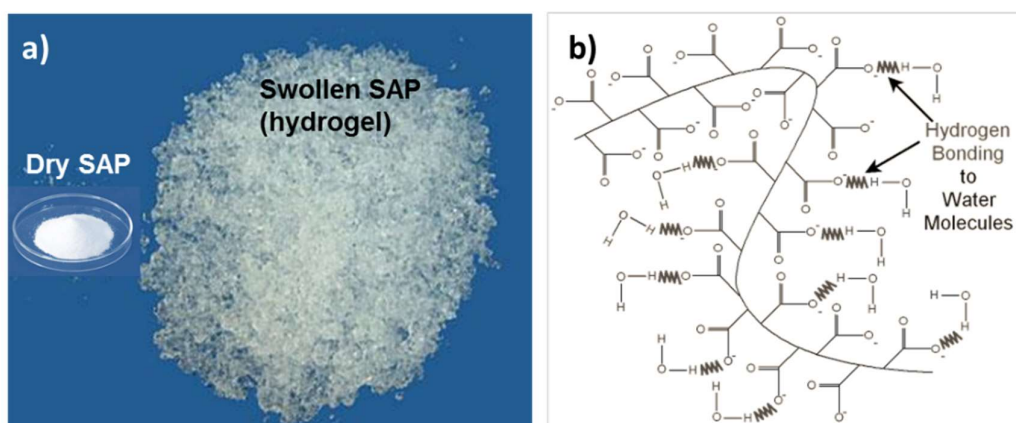
Figure 2. Superabsorbent polymer (SAP): (a) dry and swollen SAP (hydrogel), (b) molecular interactions of Na-polyacrylate.
