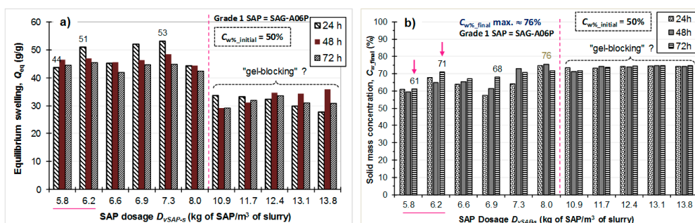
Figure 11. Tailings slurry at C_{w\%\_initial} = 50\% dewatered at different dosages of grade 1 SAP (SAG-A06P): (a) equilibrium swelling Q_{eq} for three different residence times, (b) final solids concentration C_{w\%\_final} .
