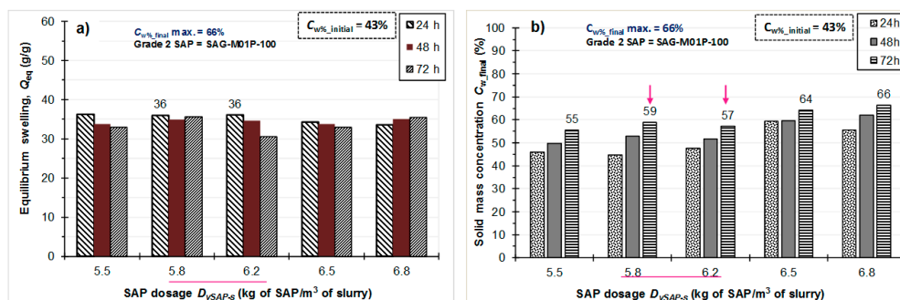
Figure 12. Tailings slurry at C_{w\%\_initial} = 43\% dewatered at different dosages of grade 2 SAP (SAG-M01P-100): (a) equilibrium swelling Q_{\text{eq}} for three different residence times, (b) final solids concentration C_{w\%\_final} .
