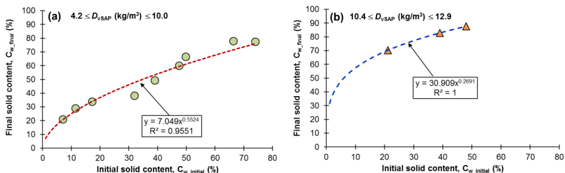
Figure 18. Power law empirical correlations between C w%_initial and C w%_final using grade 1 SAP (SAG-A06P): (a) for D vSAP-s in the range 4.2–10 kg of SAP/m 3 of slurry, (b) for D vSAP-s in the range 10.4–12.9 kg of SAP/m 3 of slurry.
