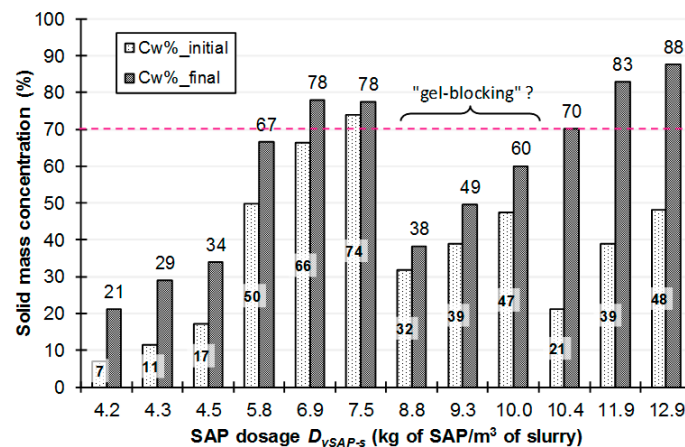
Figure 13. Results of tailings slurry dewatering using D_{vSAP-s} in the range 4.2–12.9 kg/m 3 of grade 1 SAP and after 72 h residence time.
