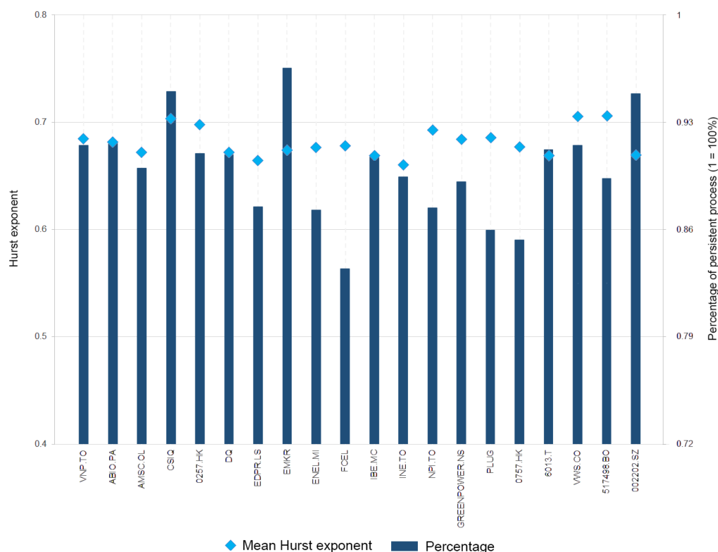
Figure 1. Mean Hurst exponents (H) and the percentage of persistent process occurrence of each component stock throughout the sample period. Random walk (efficient market) is when H = 0.5 . Persistence (trend-reinforcing) is when 0.5 < H < 1.0 , while anti-persistence (mean-reverting, cycling or contrarian) is when 0 \leq H < 0.5 .
