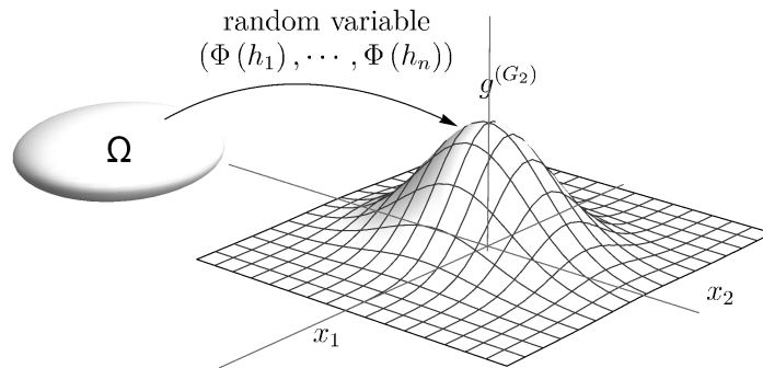
Figure 1. The multivariate Gaussian (\Phi(h_1), \dots, \Phi(h_n)) and its distribution. The Gaussian with Gramian matrix (Gram matrix) G_n, n = 2 .
