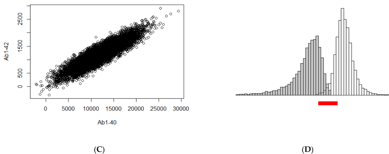
Figure 2. Illustration of the theoretical derivation with simulated data: (A) Histogram of the distribution of A\beta_{1-42} in AD (gray) and Controls (white) with obvious overlap marked by a red bar; (B) Histogram of the (overlapping) distribution of A\beta_{1-40} in AD and Controls; (C) Scatterplot of A\beta_{1-42} and A\beta_{1-40} ; (D) Histogram of the quotient of the two variables (i.e., A\beta_{42/40} ) in AD (gray) and Controls (white); obviously much smaller overlap of the two distributions, compared to that on Figure 2A, is seen (red bar). Further, both distributions are clearly denser around their respective expectations, due to the smaller dispersion.
