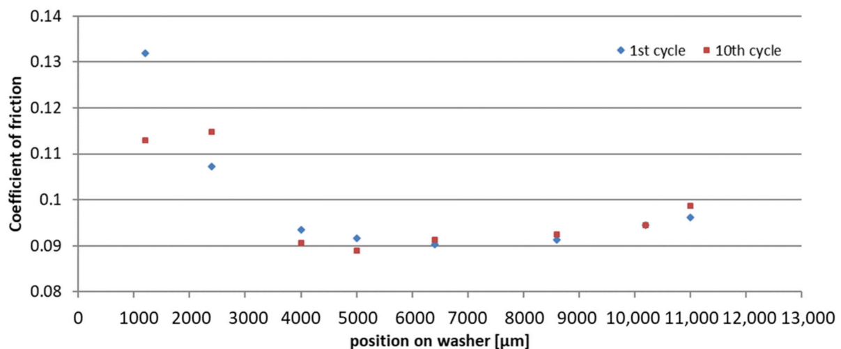
Figure 26. Coefficient of friction on the surface for the bearing washer TB 60-80 (60 kN load, 80 °C).
