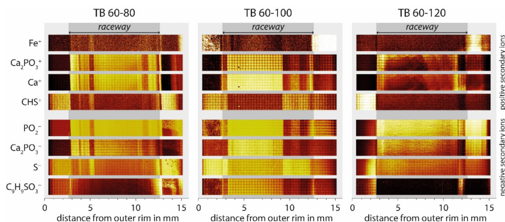
Figure 28. Distribution of selected positive (top) and negative (bottom) secondary ions obtained from large area mappings of the washer surfaces of test bearings TB 60-80 (left), TB 60-100 (middle), and TB 60-120 (right).
