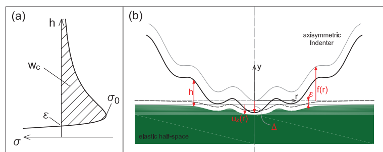
Figure 2. (a) Lennard–Jones interaction law. (b) Equivalent representation of the considered contact problem in the undeformed configuration (grey lines) and after applying a certain remote displacement \Delta (black lines).
