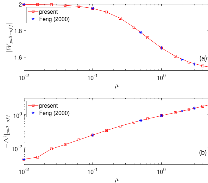
Figure 4. (a) Pull-off force |\overline{W}|_{pull-off} and (b) approach -\Delta^+_{pull-off} at pull-off as a function of the Tabor parameter \mu = [10^{-2}, 5] . Red squares were obtained with the presented Boundary Element Method (BEM) scheme, while blue asterisks were obtained from Feng [36].
