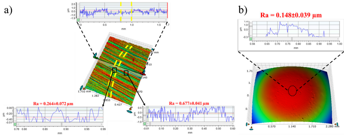
Figure S4: 3D image and scanning profile of the disc (a) and ball (b) wear track of ZDDP+Ni tribotest.
