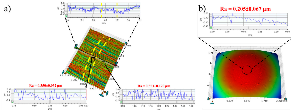
Figure S5: 3D image and scanning profile of the disc (a) and ball (b) wear track of ZDDP+CPCa tribotest.
