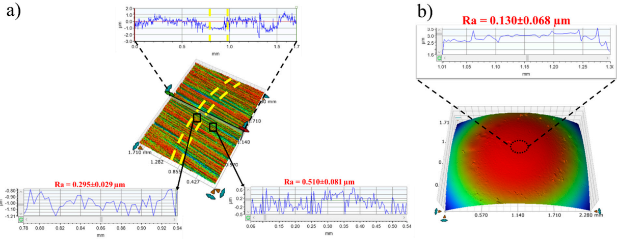
Figure S1: 3D image and scanning profile of the disc (a) and ball (b) wear track of ZDDP tribotest.
