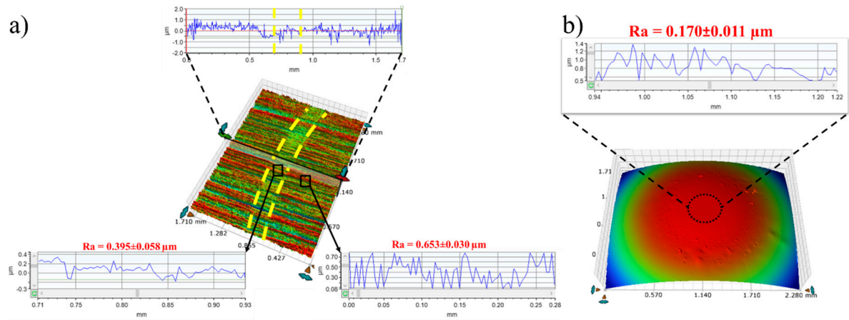
Figure S2: 3D image and scanning profile of the disc (a) and ball (b) wear track of pure CPCa tribotest.
