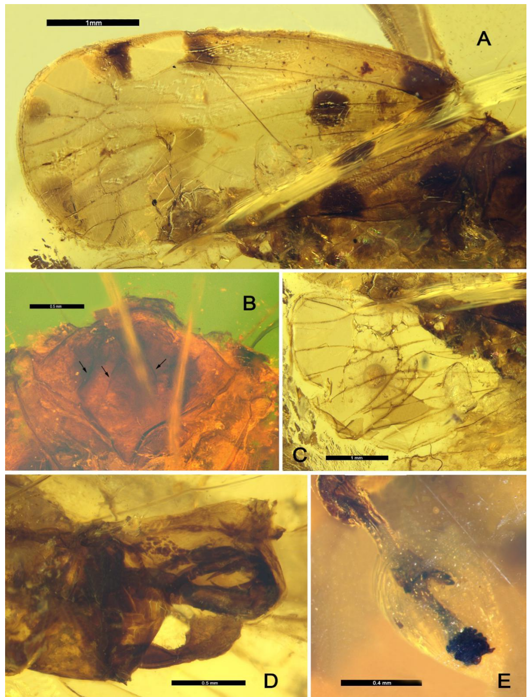
Figure 2. Maculixius jiewenae sp. nov., Holotype, MDHP11. (A) Left forewing, dorsal view. (B) Mesonotum, dorsal view. (C) Hindwing, dorsal view. (D) Male terminalia, lateral view. (E) Apex of tibia and tarsus on left leg, ventral view. The arrows indicate the visible carinae.
